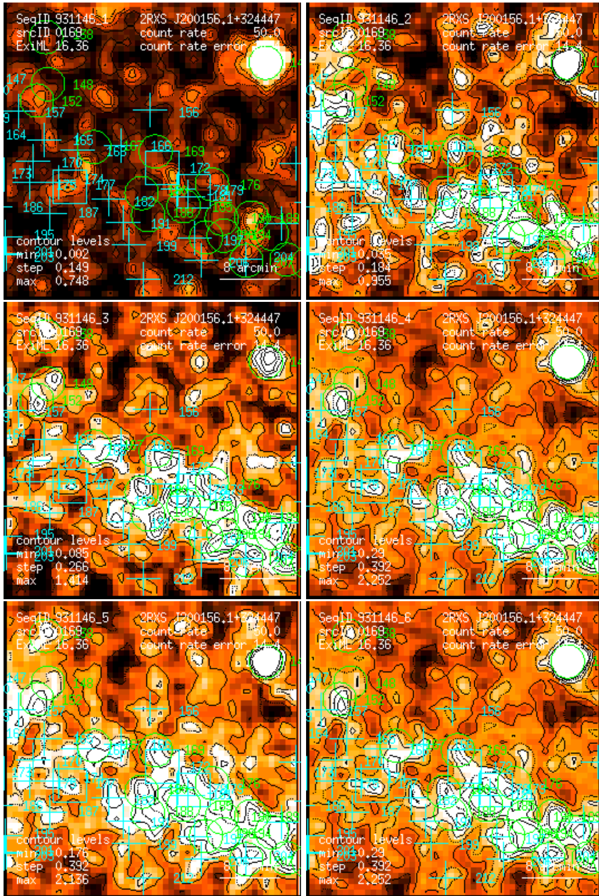
Figure 169: RASS 931146: detection 0169: band rate images, Gaussian filter: (1) PSPC channels 11 – 41, (2) 52 – 90, (3) 91 – 201, (4) 11 – 235, (5) 52 – 201, (6) 11 – 201. Broad band rates in counts/ks. Band rate contour levels in counts/ks/arcmin 2 .
