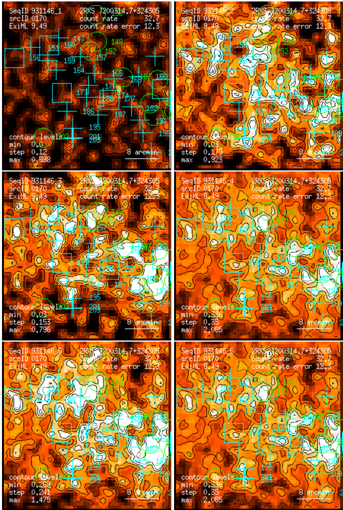
Figure 170: RASS 931146: detection 0170: band rate images, Gaussian filter: (1) PSPC channels 11 – 41, (2) 52 – 90, (3) 91 – 201, (4) 11 – 235, (5) 52 – 201, (6) 11 – 201. Broad band rates in counts/ks. Band rate contour levels in counts/ks/arcmin 2 .
