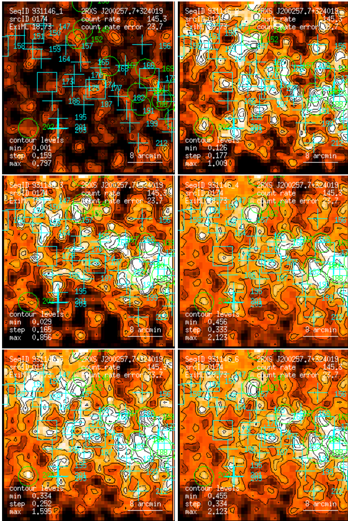
Figure 174: RASS 931146: detection 0174: band rate images, Gaussian filter: (1) PSPC channels 11 – 41, (2) 52 – 90, (3) 91 – 201, (4) 11 – 235, (5) 52 – 201, (6) 11 – 201. Broad band rates in counts/ks. Band rate contour levels in counts/ks/arcmin 2 .
