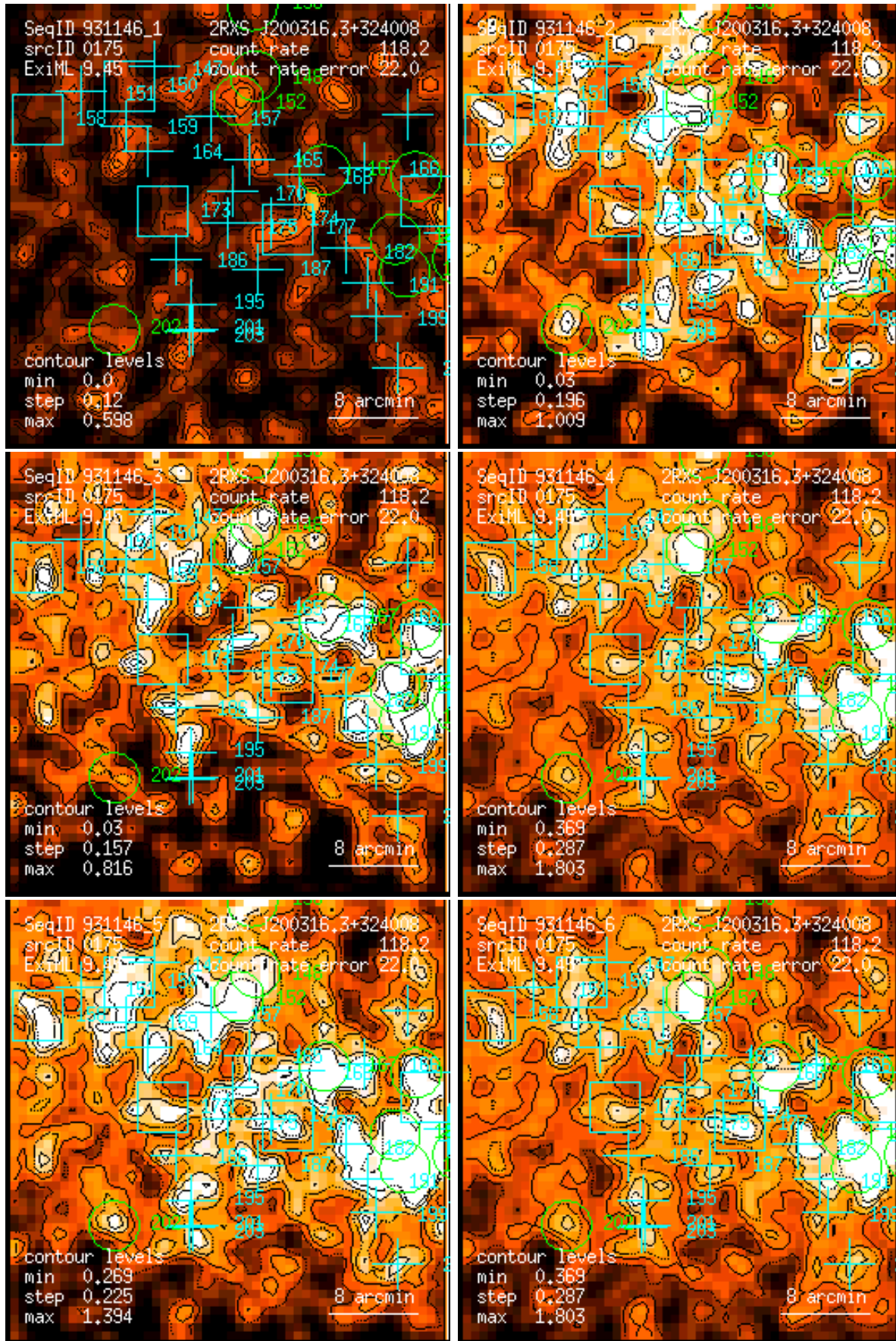
Figure 175: RASS 931146: detection 0175: band rate images, Gaussian filter: (1) PSPC channels 11 – 41, (2) 52 – 90, (3) 91 – 201, (4) 11 – 235, (5) 52 – 201, (6) 11 – 201. Broad band rates in counts/ks. Band rate contour levels in counts/ks/arcmin 2 .
