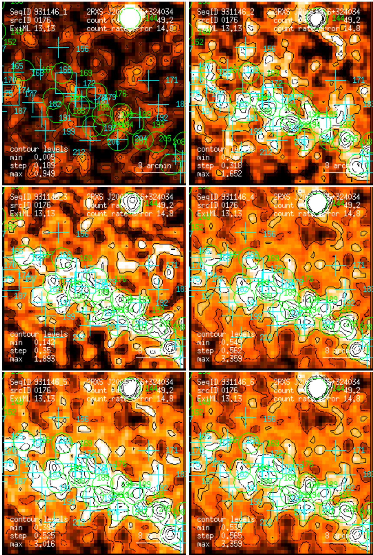
Figure 176: RASS 931146: detection 0176: band rate images, Gaussian filter: (1) PSPC channels 11 – 41, (2) 52 – 90, (3) 91 – 201, (4) 11 – 235, (5) 52 – 201, (6) 11 – 201. Broad band rates in counts/ks. Band rate contour levels in counts/ks/arcmin 2 .
