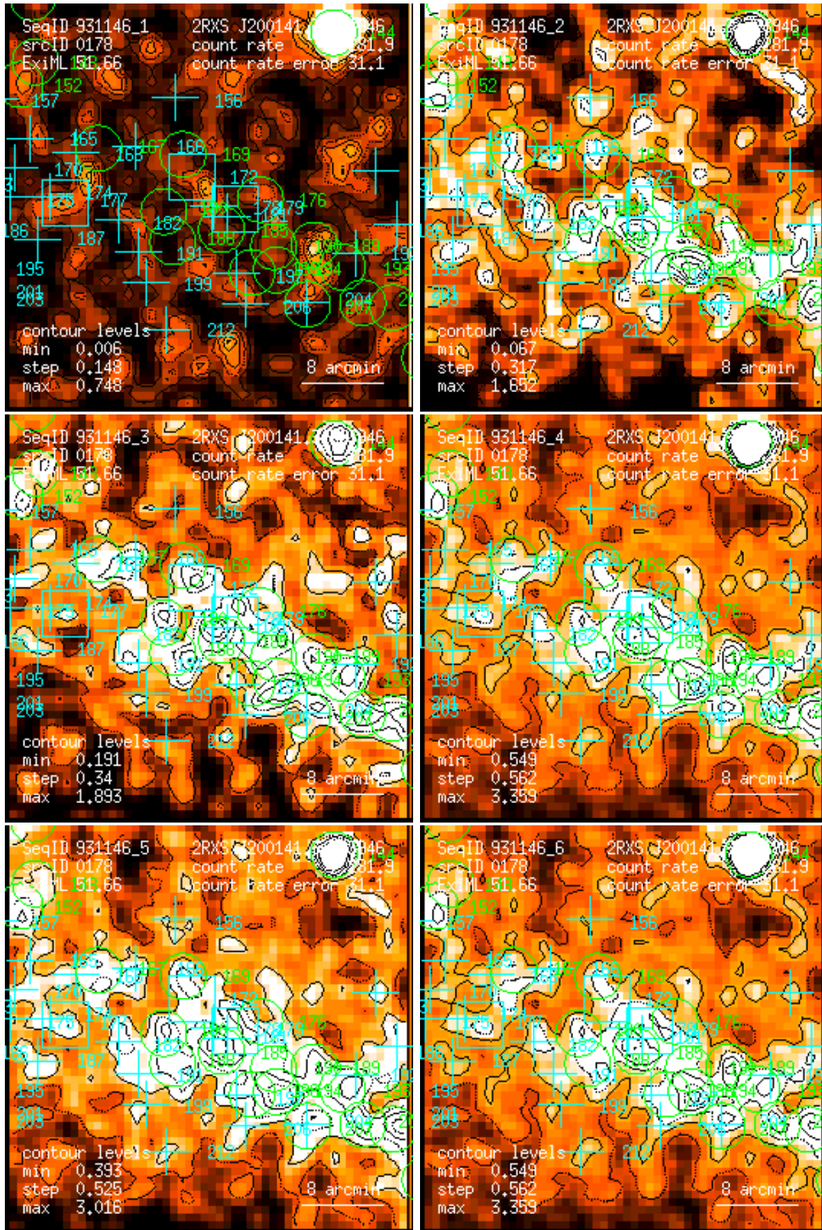
Figure 178: RASS 931146: detection 0178: band rate images, Gaussian filter: (1) PSPC channels 11 – 41, (2) 52 – 90, (3) 91 – 201, (4) 11 – 235, (5) 52 – 201, (6) 11 – 201. Broad band rates in counts/ks. Band rate contour levels in counts/ks/arcmin 2 .
