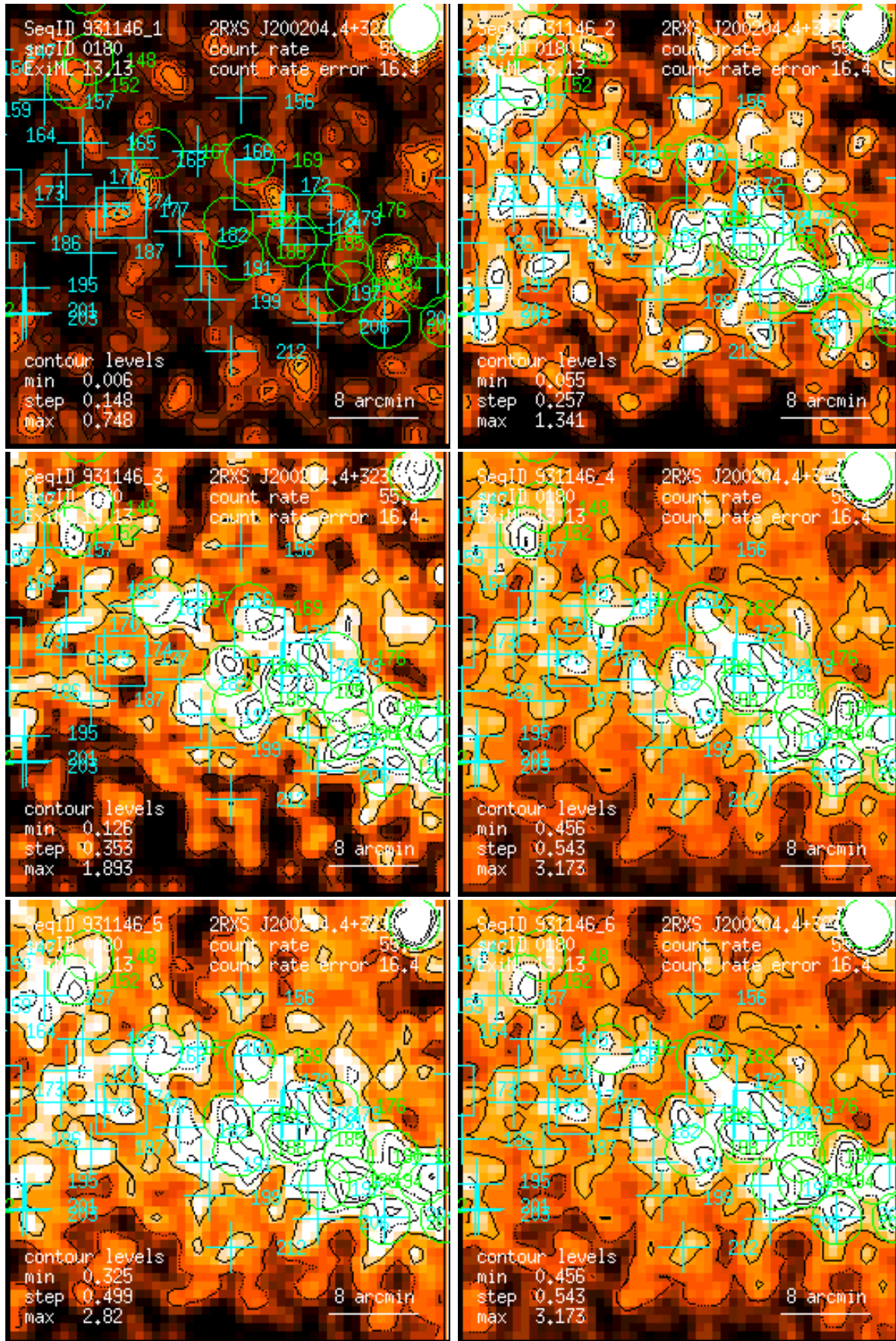
Figure 180: RASS 931146: detection 0180: band rate images, Gaussian filter: (1) PSPC channels 11 – 41, (2) 52 – 90, (3) 91 – 201, (4) 11 – 235, (5) 52 – 201, (6) 11 – 201. Broad band rates in counts/ks. Band rate contour levels in counts/ks/arcmin 2 .
