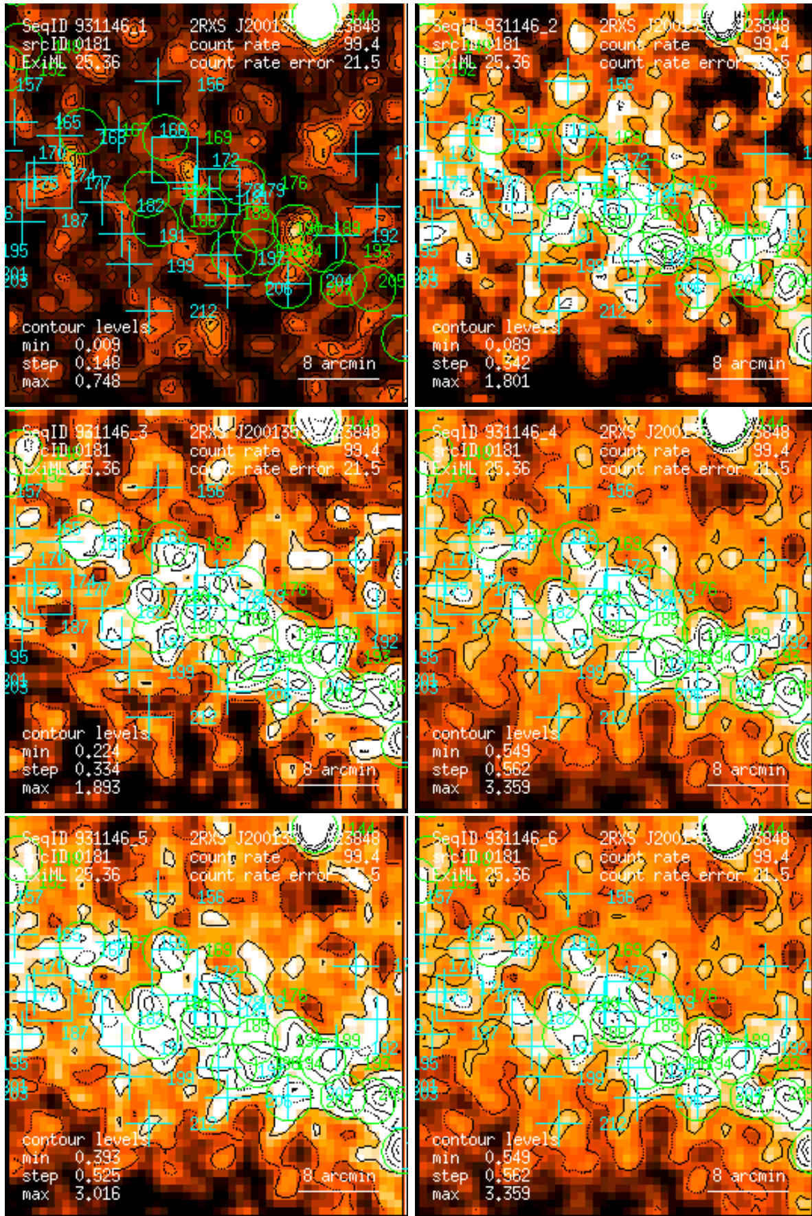
Figure 181: RASS 931146: detection 0181: band rate images, Gaussian filter: (1) PSPC channels 11 – 41, (2) 52 – 90, (3) 91 – 201, (4) 11 – 235, (5) 52 – 201, (6) 11 – 201. Broad band rates in counts/ks. Band rate contour levels in counts/ks/arcmin 2 .
