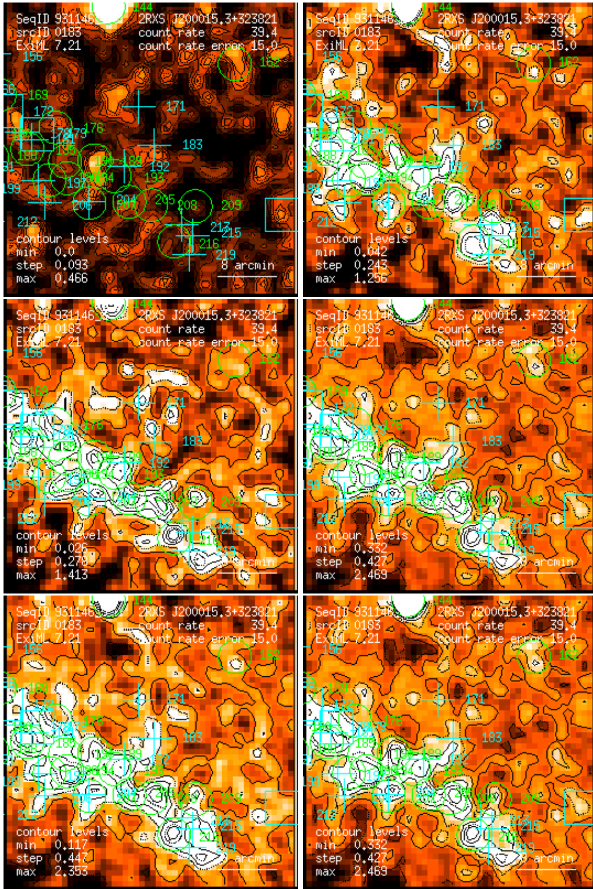
Figure 183: RASS 931146: detection 0183: band rate images, Gaussian filter: (1) PSPC channels 11 – 41, (2) 52 – 90, (3) 91 – 201, (4) 11 – 235, (5) 52 – 201, (6) 11 – 201. Broad band rates in counts/ks. Band rate contour levels in counts/ks/arcmin 2 .
