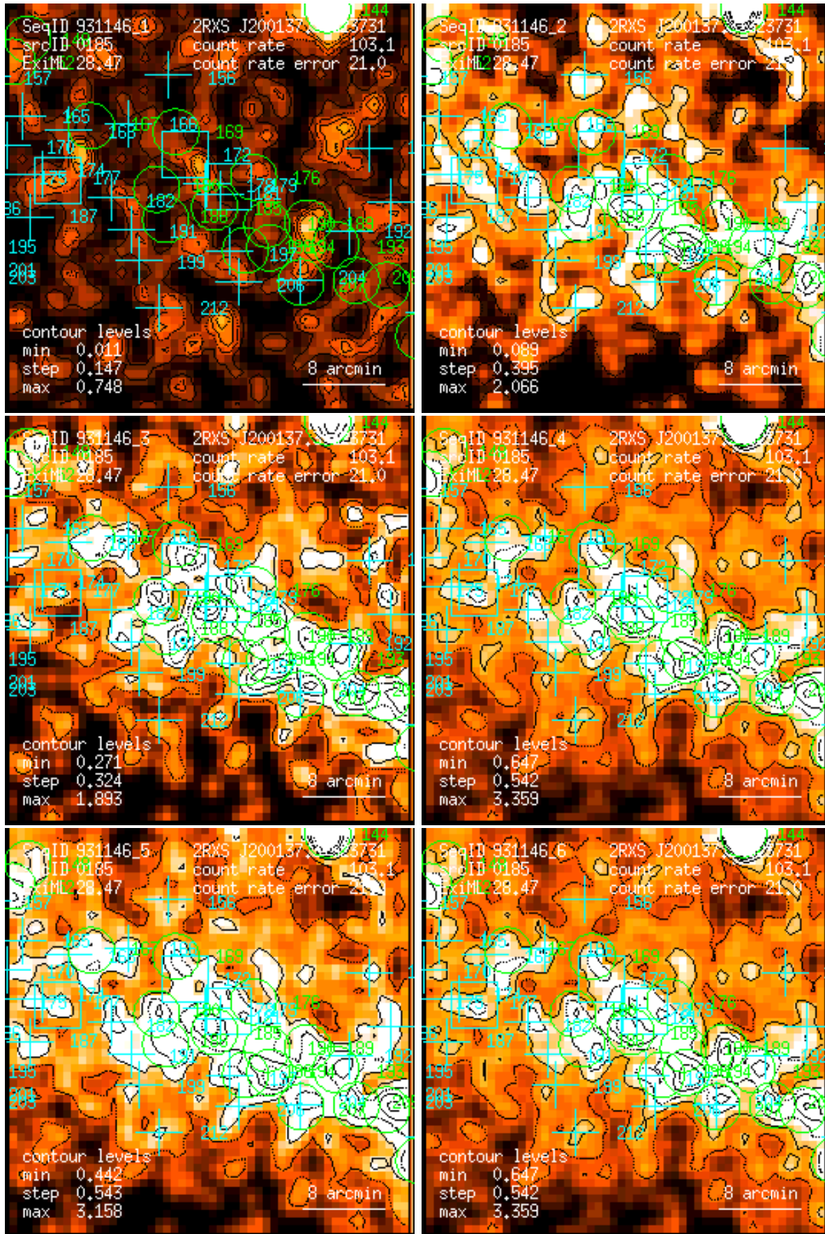
Figure 185: RASS 931146: detection 0185: band rate images, Gaussian filter: (1) PSPC channels 11 – 41, (2) 52 – 90, (3) 91 – 201, (4) 11 – 235, (5) 52 – 201, (6) 11 – 201. Broad band rates in counts/ks. Band rate contour levels in counts/ks/arcmin 2 .
