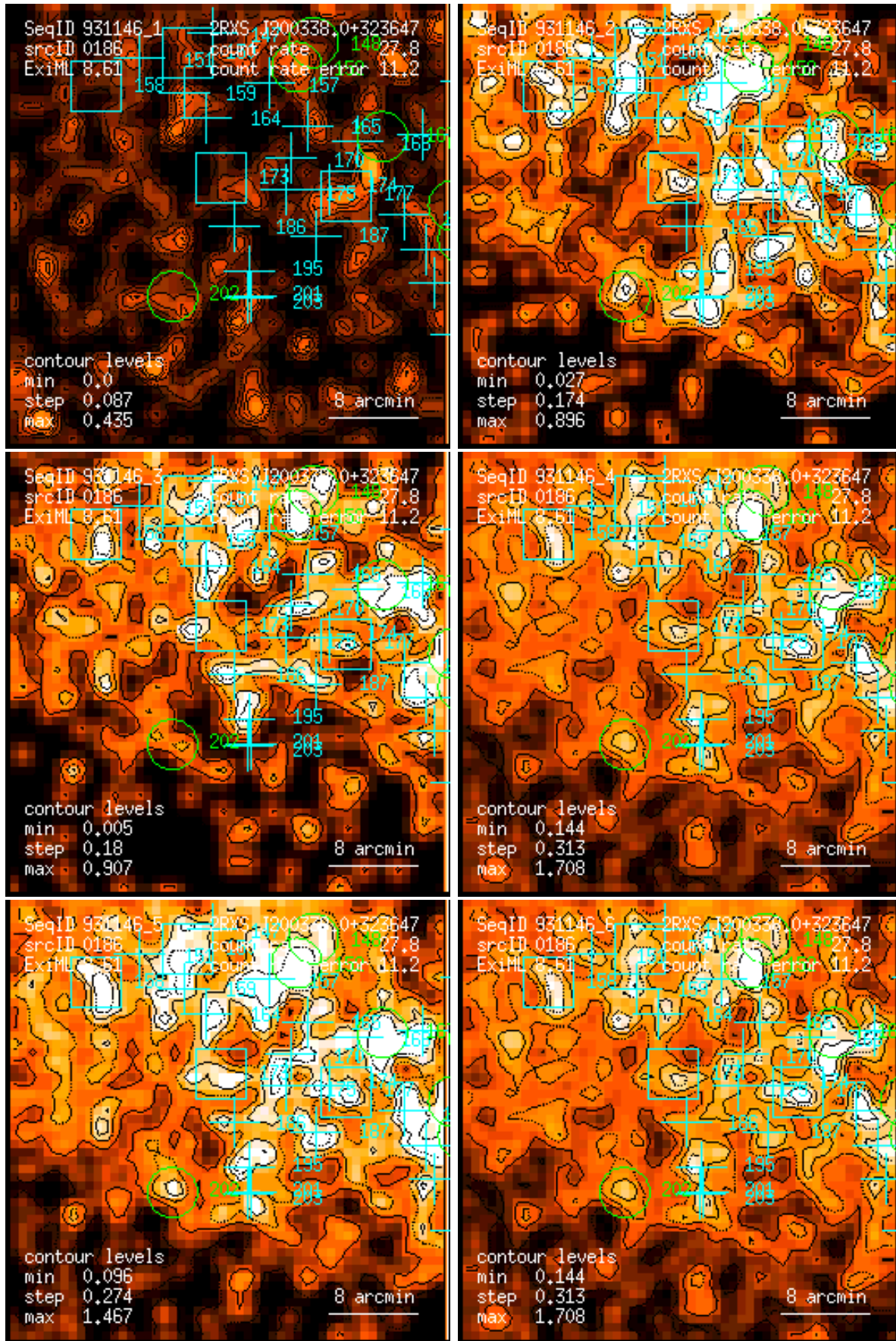
Figure 186: RASS 931146: detection 0186: band rate images, Gaussian filter: (1) PSPC channels 11 – 41, (2) 52 – 90, (3) 91 – 201, (4) 11 – 235, (5) 52 – 201, (6) 11 – 201. Broad band rates in counts/ks. Band rate contour levels in counts/ks/arcmin 2 .
