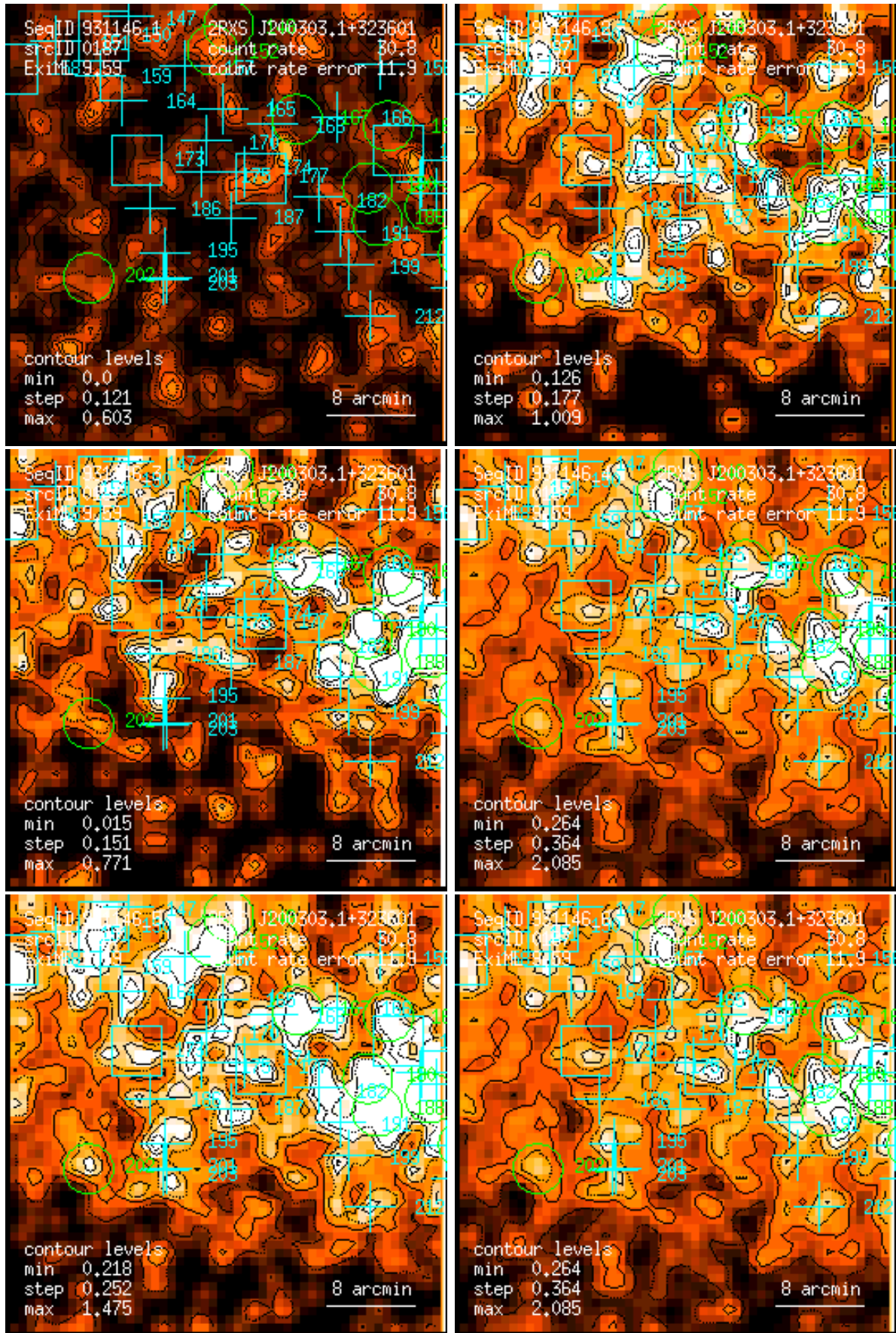
Figure 187: RASS 931146: detection 0187: band rate images, Gaussian filter: (1) PSPC channels 11 – 41, (2) 52 – 90, (3) 91 – 201, (4) 11 – 235, (5) 52 – 201, (6) 11 – 201. Broad band rates in counts/ks. Band rate contour levels in counts/ks/arcmin 2 .
