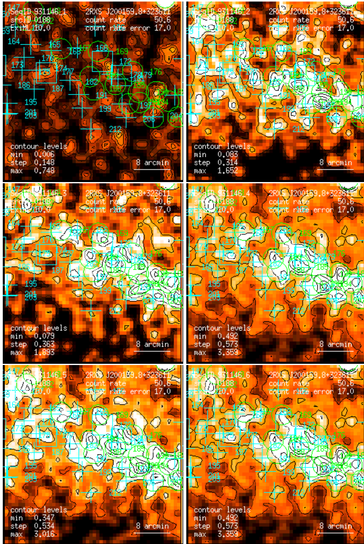
Figure 188: RASS 931146: detection 0188: band rate images, Gaussian filter: (1) PSPC channels 11 – 41, (2) 52 – 90, (3) 91 – 201, (4) 11 – 235, (5) 52 – 201, (6) 11 – 201. Broad band rates in counts/ks. Band rate contour levels in counts/ks/arcmin 2 .
