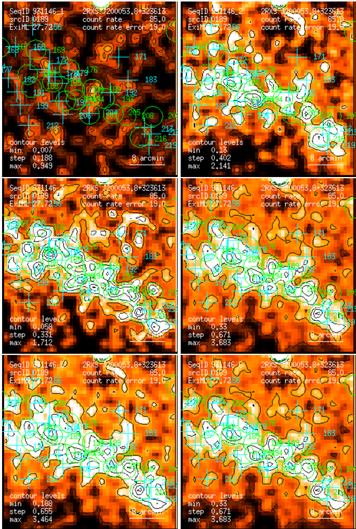
Figure 189: RASS 931146: detection 0189: band rate images, Gaussian filter: (1) PSPC channels 11 – 41, (2) 52 – 90, (3) 91 – 201, (4) 11 – 235, (5) 52 – 201, (6) 11 – 201. Broad band rates in counts/ks. Band rate contour levels in counts/ks/arcmin 2 .
