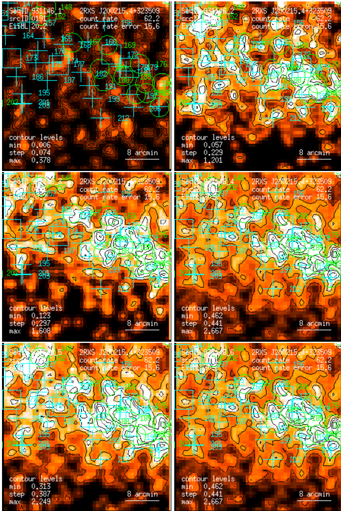
Figure 191: RASS 931146: detection 0191: band rate images, Gaussian filter: (1) PSPC channels 11 – 41, (2) 52 – 90, (3) 91 – 201, (4) 11 – 235, (5) 52 – 201, (6) 11 – 201. Broad band rates in counts/ks. Band rate contour levels in counts/ks/arcmin 2 .
