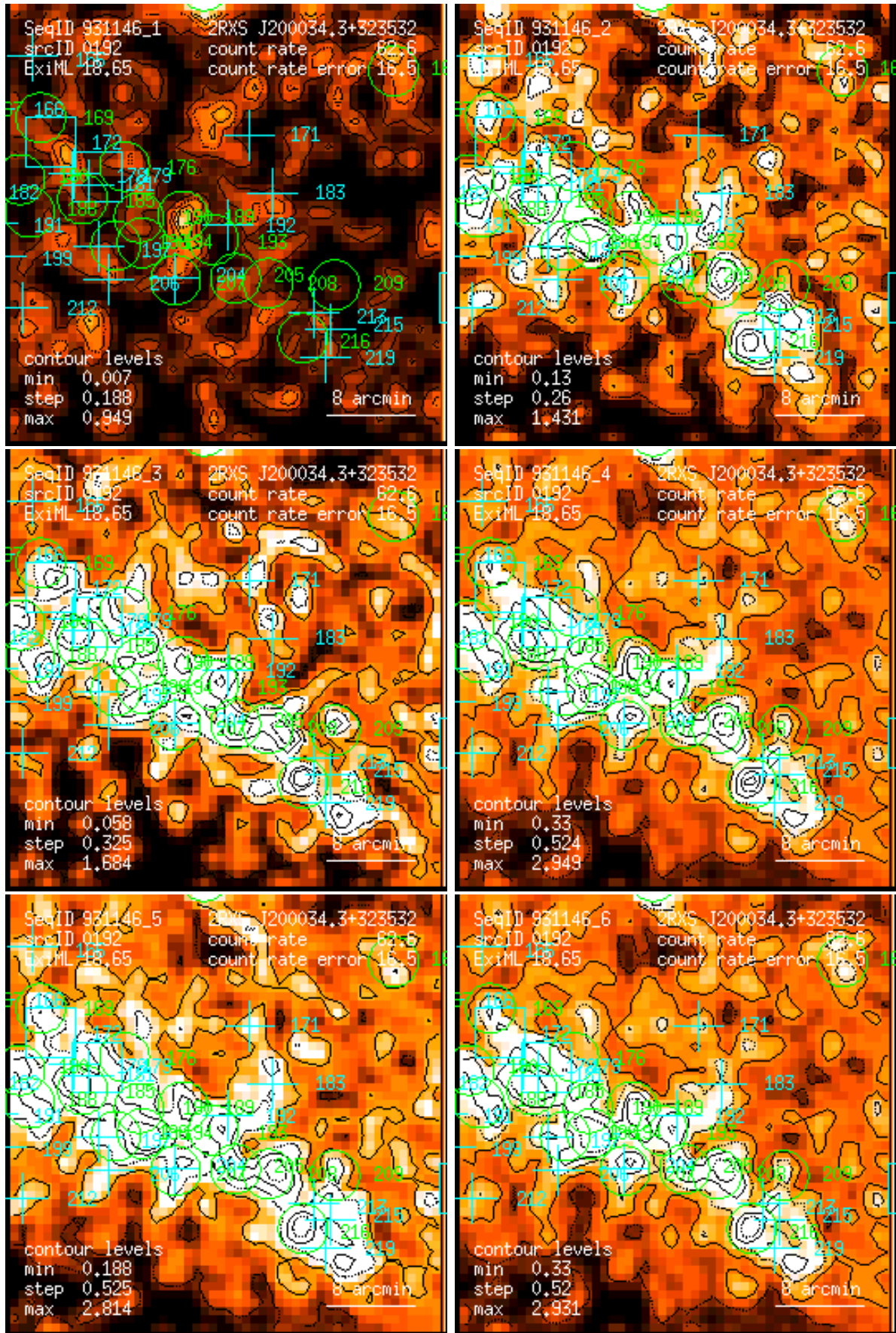
Figure 192: RASS 931146: detection 0192: band rate images, Gaussian filter: (1) PSPC channels 11 – 41, (2) 52 – 90, (3) 91 – 201, (4) 11 – 235, (5) 52 – 201, (6) 11 – 201. Broad band rates in counts/ks. Band rate contour levels in counts/ks/arcmin 2 .
