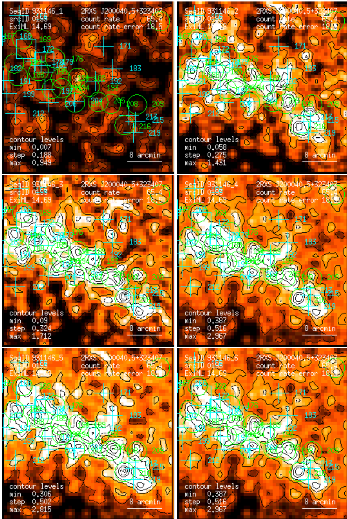
Figure 193: RASS 931146: detection 0193: band rate images, Gaussian filter: (1) PSPC channels 11 – 41, (2) 52 – 90, (3) 91 – 201, (4) 11 – 235, (5) 52 – 201, (6) 11 – 201. Broad band rates in counts/ks. Band rate contour levels in counts/ks/arcmin 2 .
