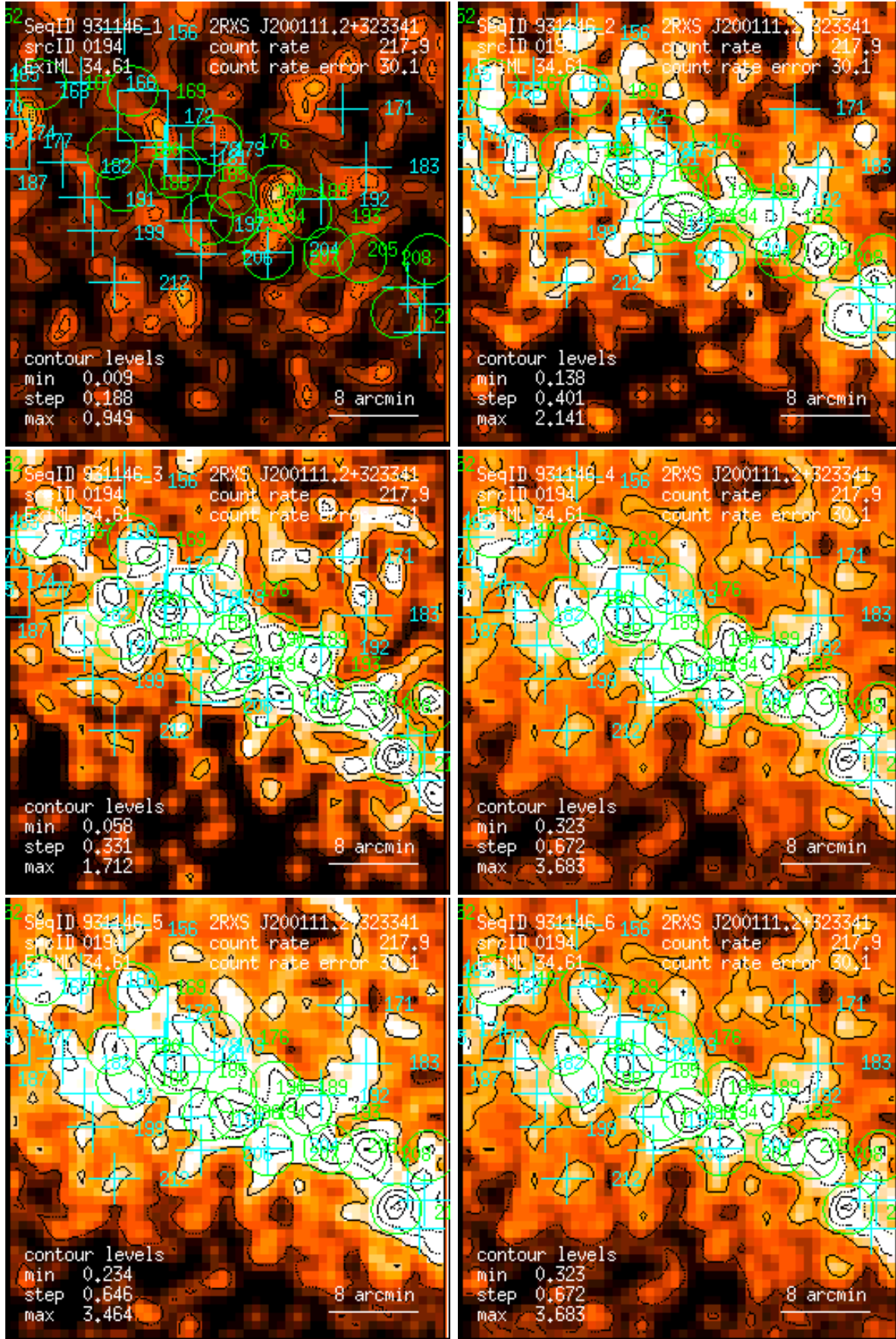
Figure 194: RASS 931146: detection 0194: band rate images, Gaussian filter: (1) PSPC channels 11 – 41, (2) 52 – 90, (3) 91 – 201, (4) 11 – 235, (5) 52 – 201, (6) 11 – 201. Broad band rates in counts/ks. Band rate contour levels in counts/ks/arcmin 2 .
