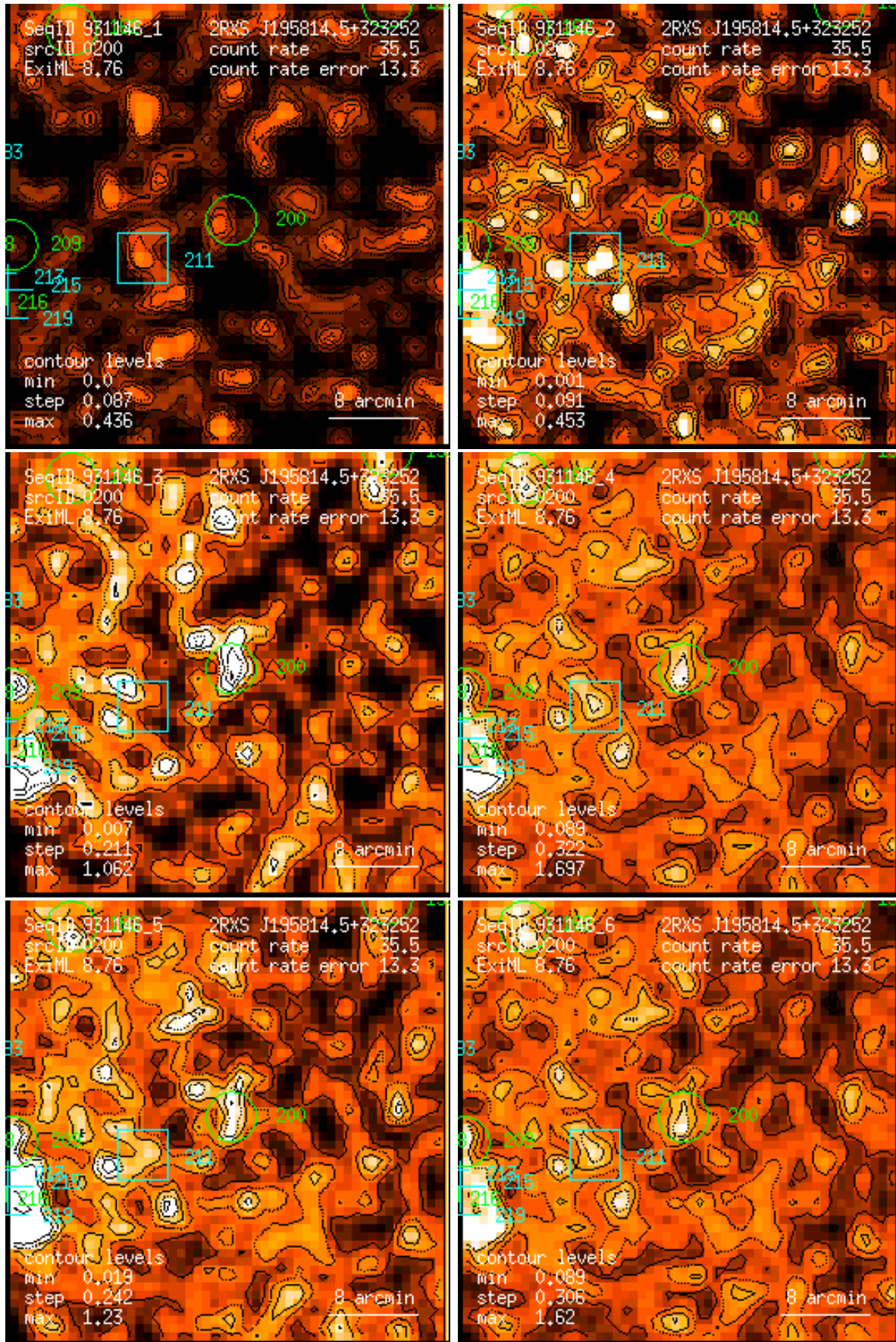
Figure 200: RASS 931146: detection 0200: band rate images, Gaussian filter: (1) PSPC channels 11 – 41, (2) 52 – 90, (3) 91 – 201, (4) 11 – 235, (5) 52 – 201, (6) 11 – 201. Broad band rates in counts/ks. Band rate contour levels in counts/ks/arcmin 2 .
