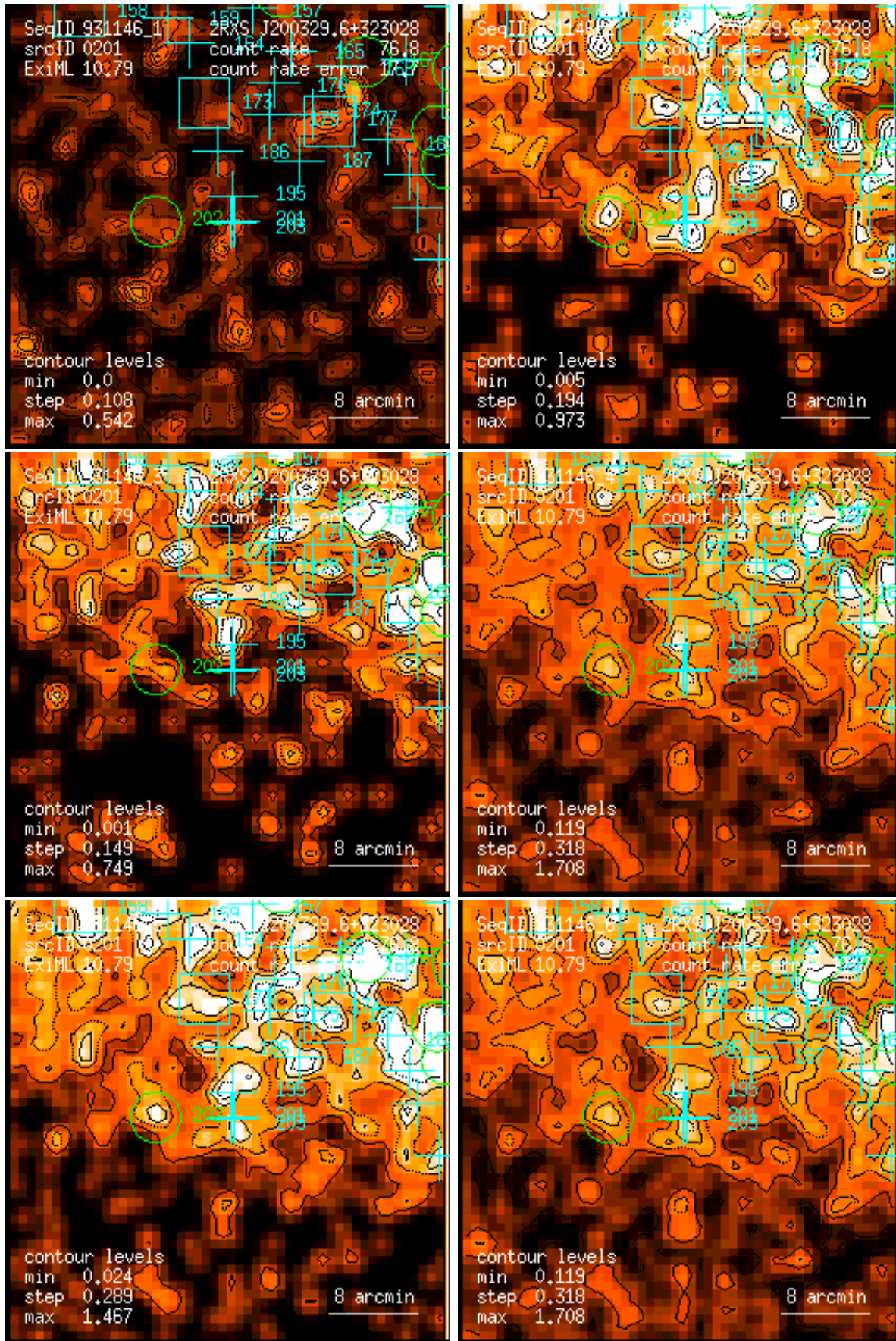
Figure 201: RASS 931146: detection 0201: band rate images, Gaussian filter: (1) PSPC channels 11 – 41, (2) 52 – 90, (3) 91 – 201, (4) 11 – 235, (5) 52 – 201, (6) 11 – 201. Broad band rates in counts/ks. Band rate contour levels in counts/ks/arcmin 2 .
