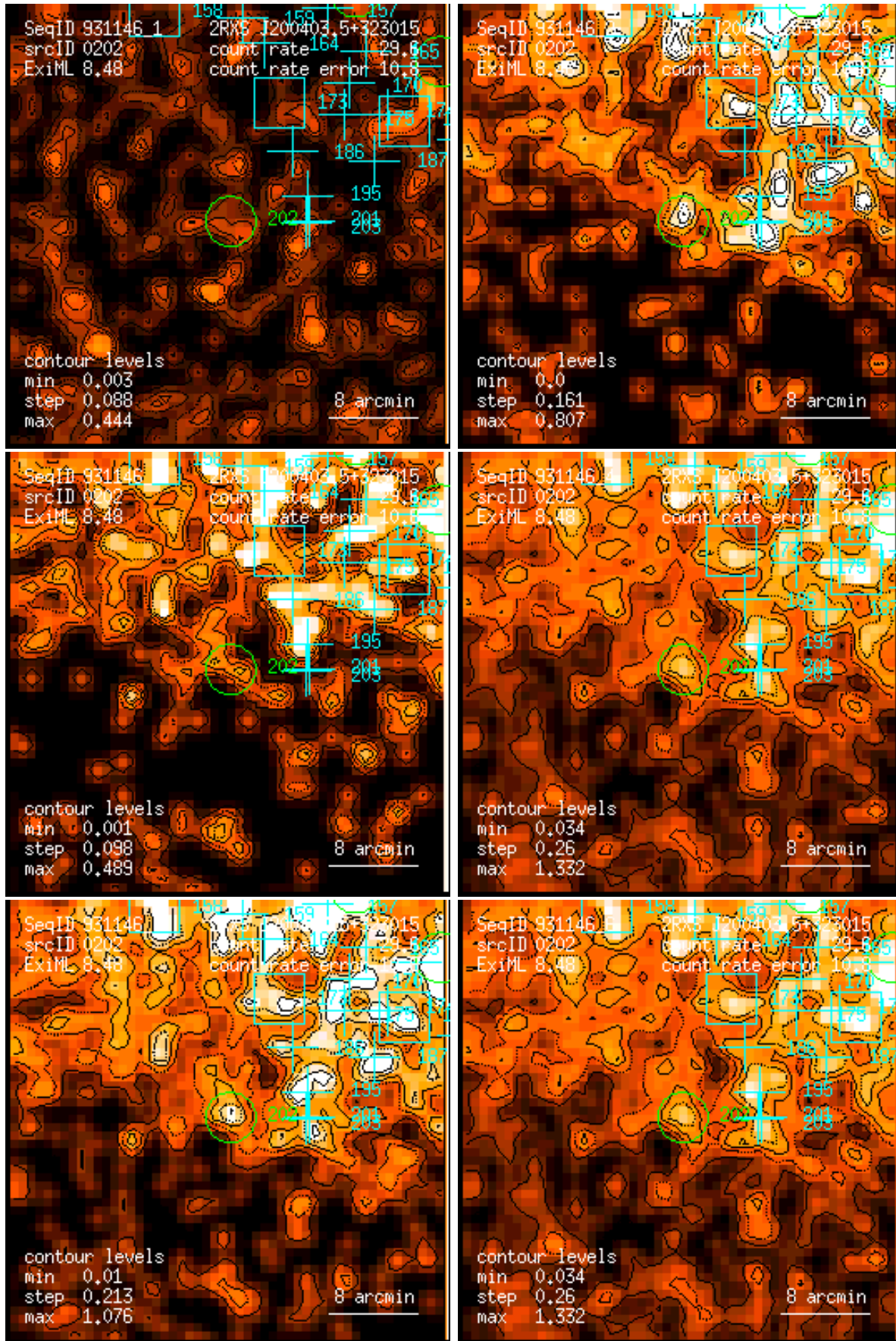
Figure 202: RASS 931146: detection 0202: band rate images, Gaussian filter: (1) PSPC channels 11 – 41, (2) 52 – 90, (3) 91 – 201, (4) 11 – 235, (5) 52 – 201, (6) 11 – 201. Broad band rates in counts/ks. Band rate contour levels in counts/ks/arcmin 2 .
