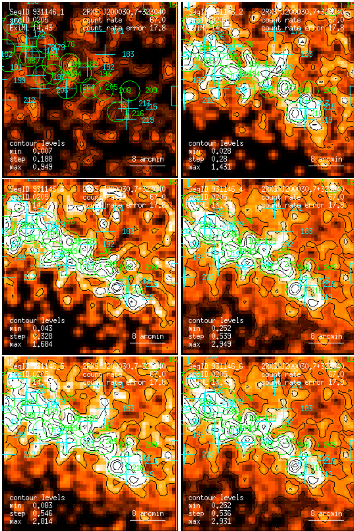
Figure 205: RASS 931146: detection 0205: band rate images, Gaussian filter: (1) PSPC channels 11 – 41, (2) 52 – 90, (3) 91 – 201, (4) 11 – 235, (5) 52 – 201, (6) 11 – 201. Broad band rates in counts/ks. Band rate contour levels in counts/ks/arcmin 2 .
