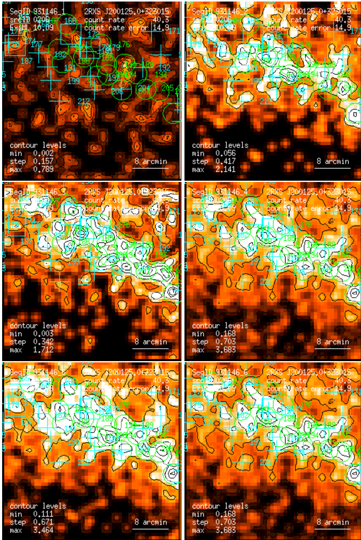
Figure 206: RASS 931146: detection 0206: band rate images, Gaussian filter: (1) PSPC channels 11 – 41, (2) 52 – 90, (3) 91 – 201, (4) 11 – 235, (5) 52 – 201, (6) 11 – 201. Broad band rates in counts/ks. Band rate contour levels in counts/ks/arcmin 2 .
