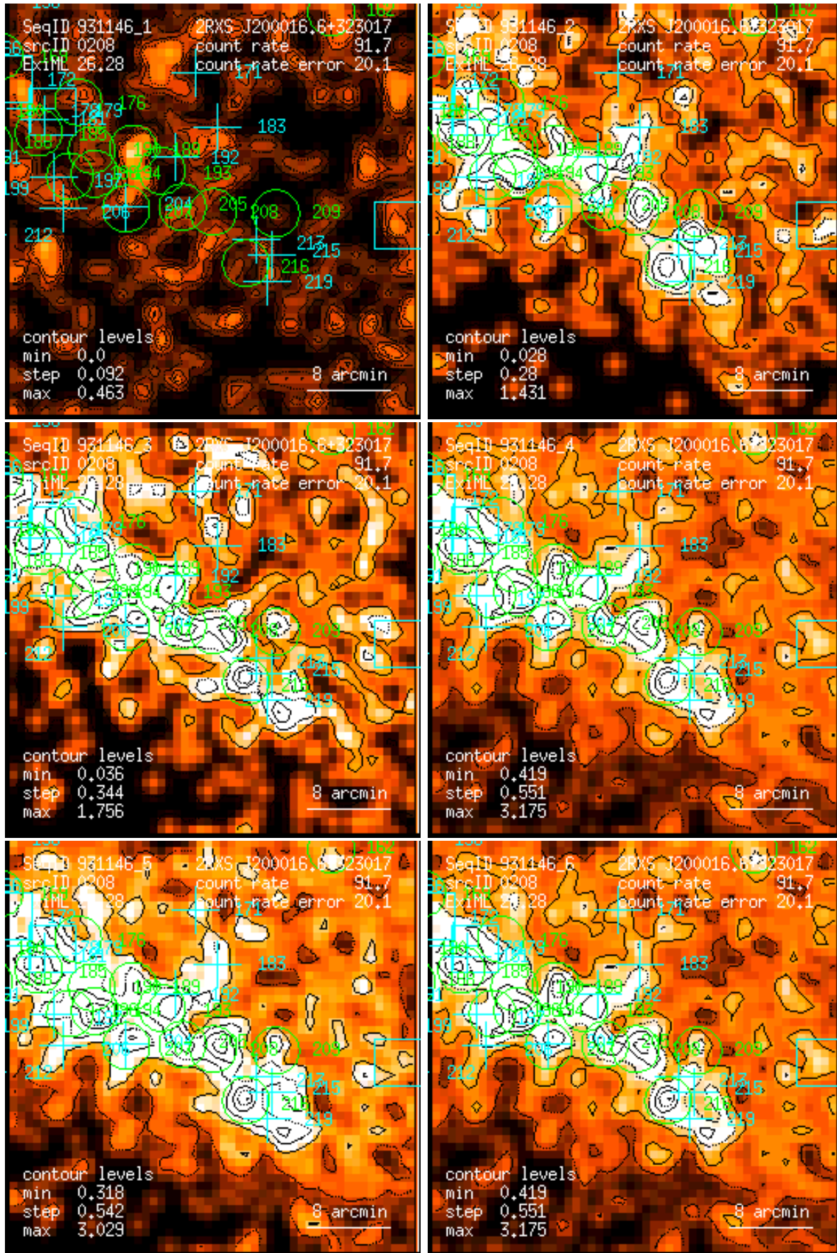
Figure 208: RASS 931146: detection 0208: band rate images, Gaussian filter: (1) PSPC channels 11 – 41, (2) 52 – 90, (3) 91 – 201, (4) 11 – 235, (5) 52 – 201, (6) 11 – 201. Broad band rates in counts/ks. Band rate contour levels in counts/ks/arcmin 2 .
