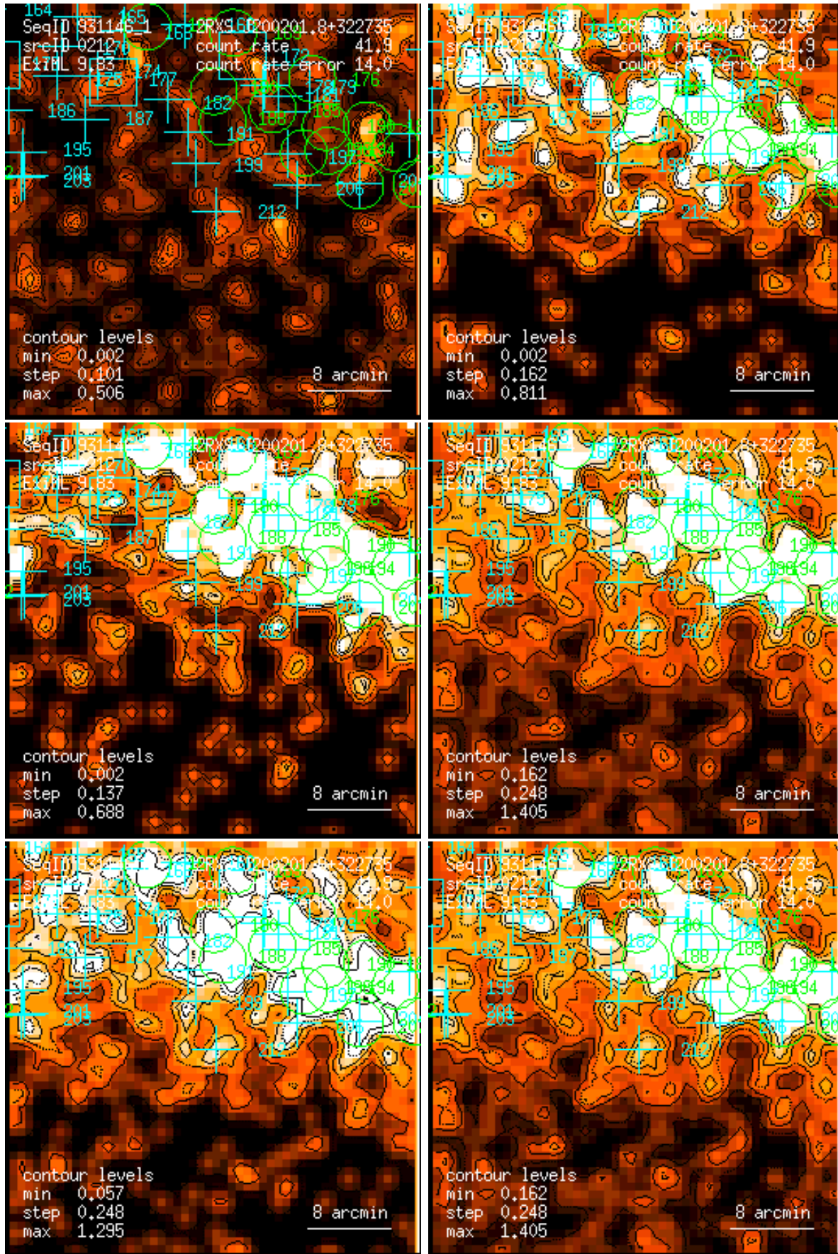
Figure 212: RASS 931146: detection 0212: band rate images, Gaussian filter: (1) PSPC channels 11 – 41, (2) 52 – 90, (3) 91 – 201, (4) 11 – 235, (5) 52 – 201, (6) 11 – 201. Broad band rates in counts/ks. Band rate contour levels in counts/ks/arcmin 2 .
