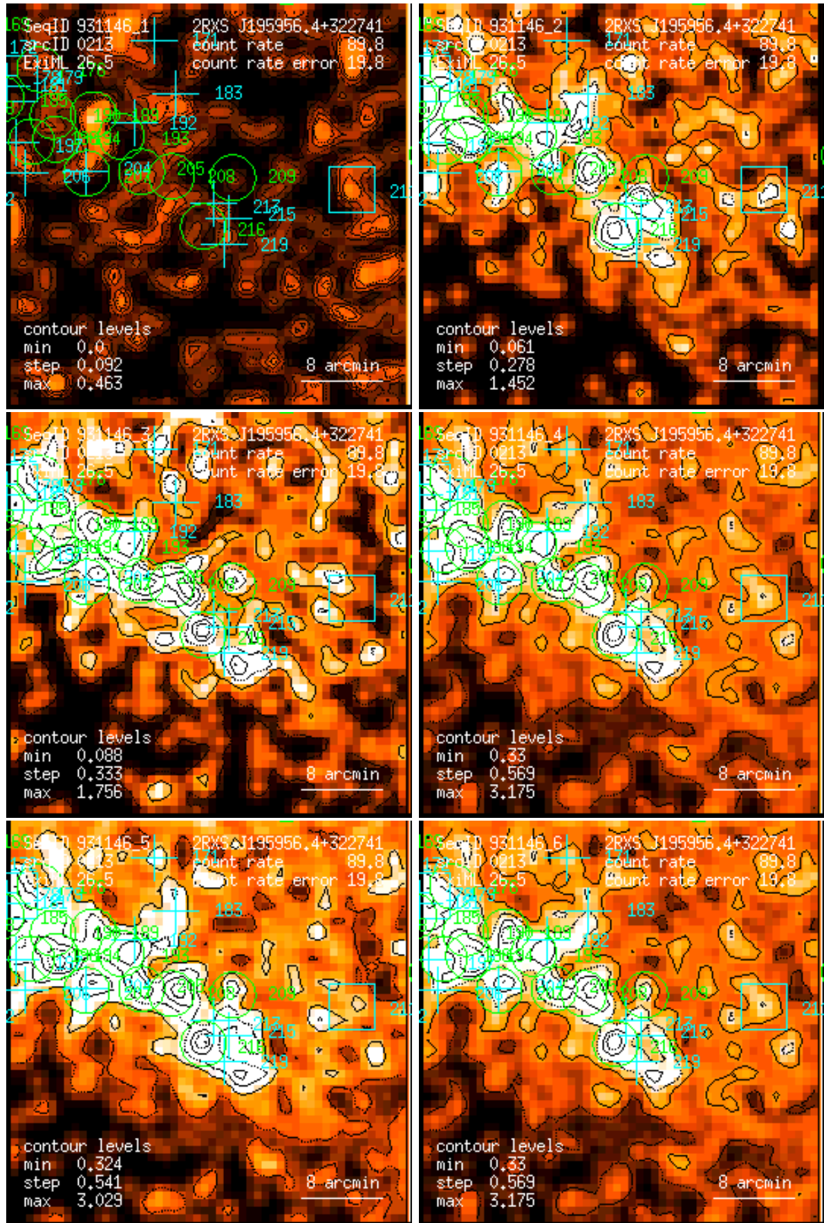
Figure 213: RASS 931146: detection 0213: band rate images, Gaussian filter: (1) PSPC channels 11 – 41, (2) 52 – 90, (3) 91 – 201, (4) 11 – 235, (5) 52 – 201, (6) 11 – 201. Broad band rates in counts/ks. Band rate contour levels in counts/ks/arcmin 2 .
