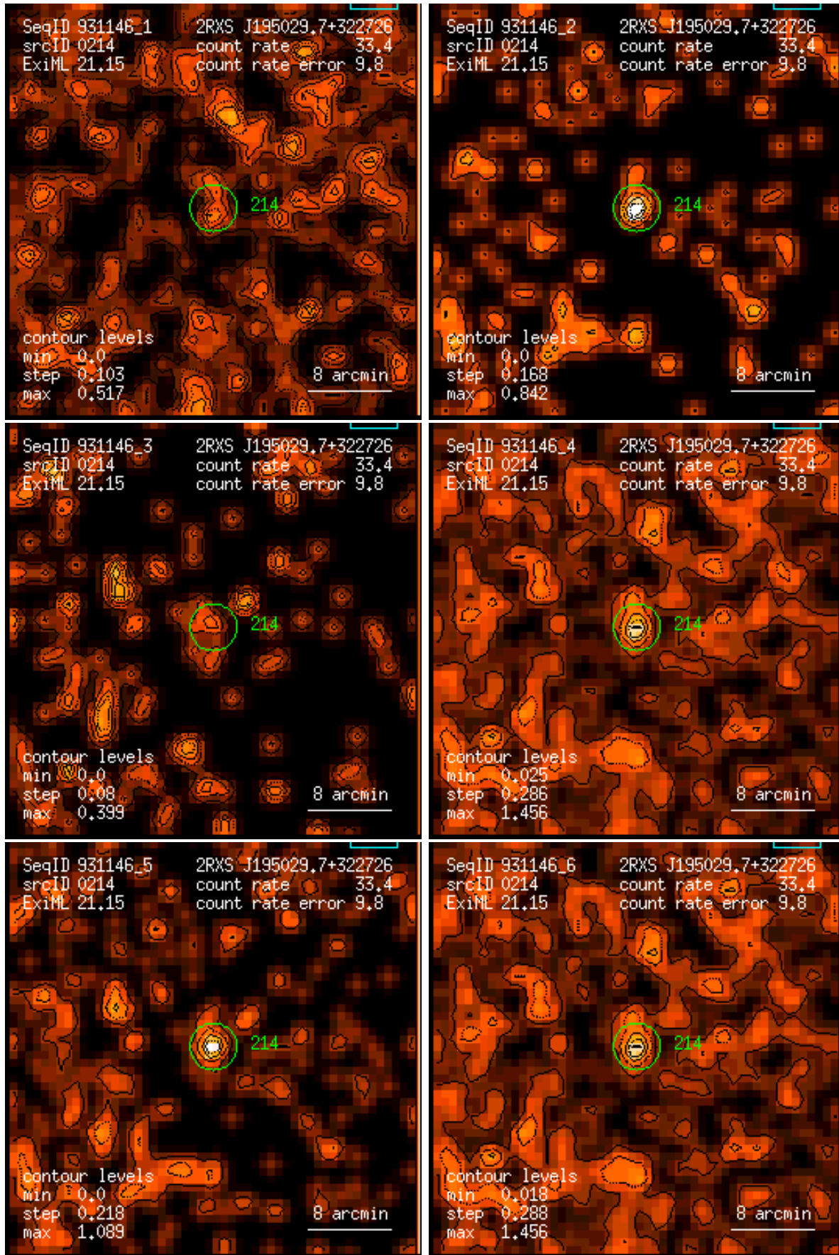
Figure 214: RASS 931146: detection 0214: band rate images, Gaussian filter: (1) PSPC channels 11 – 41, (2) 52 – 90, (3) 91 – 201, (4) 11 – 235, (5) 52 – 201, (6) 11 – 201. Broad band rates in counts/ks. Band rate contour levels in counts/ks/arcmin 2 .
