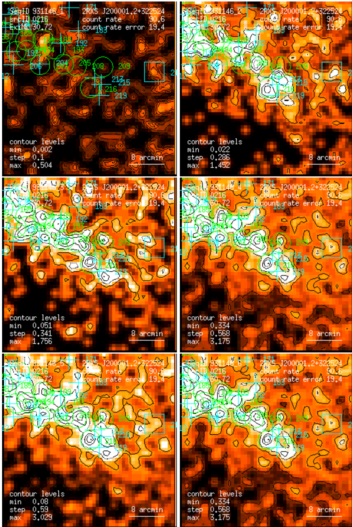
Figure 216: RASS 931146: detection 0216: band rate images, Gaussian filter: (1) PSPC channels 11 – 41, (2) 52 – 90, (3) 91 – 201, (4) 11 – 235, (5) 52 – 201, (6) 11 – 201. Broad band rates in counts/ks. Band rate contour levels in counts/ks/arcmin 2 .
