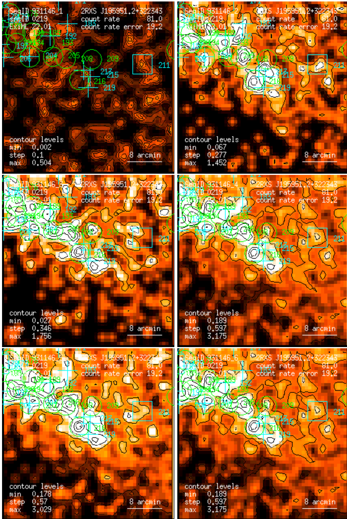
Figure 219: RASS 931146: detection 0219: band rate images, Gaussian filter: (1) PSPC channels 11 – 41, (2) 52 – 90, (3) 91 – 201, (4) 11 – 235, (5) 52 – 201, (6) 11 – 201. Broad band rates in counts/ks. Band rate contour levels in counts/ks/arcmin 2 .
