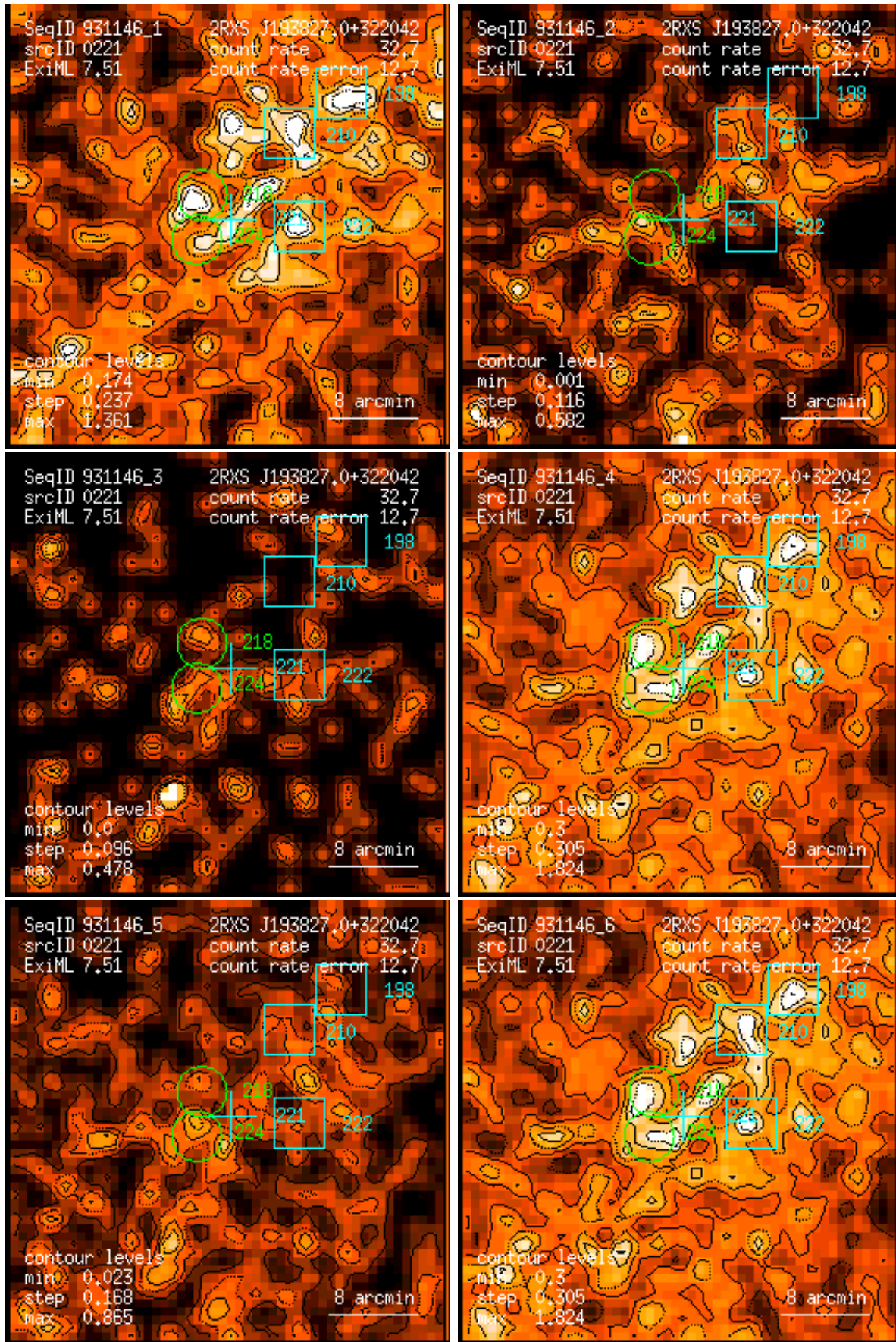
Figure 221: RASS 931146: detection 0221: band rate images, Gaussian filter: (1) PSPC channels 11 – 41, (2) 52 – 90, (3) 91 – 201, (4) 11 – 235, (5) 52 – 201, (6) 11 – 201. Broad band rates in counts/ks. Band rate contour levels in counts/ks/arcmin 2 .
