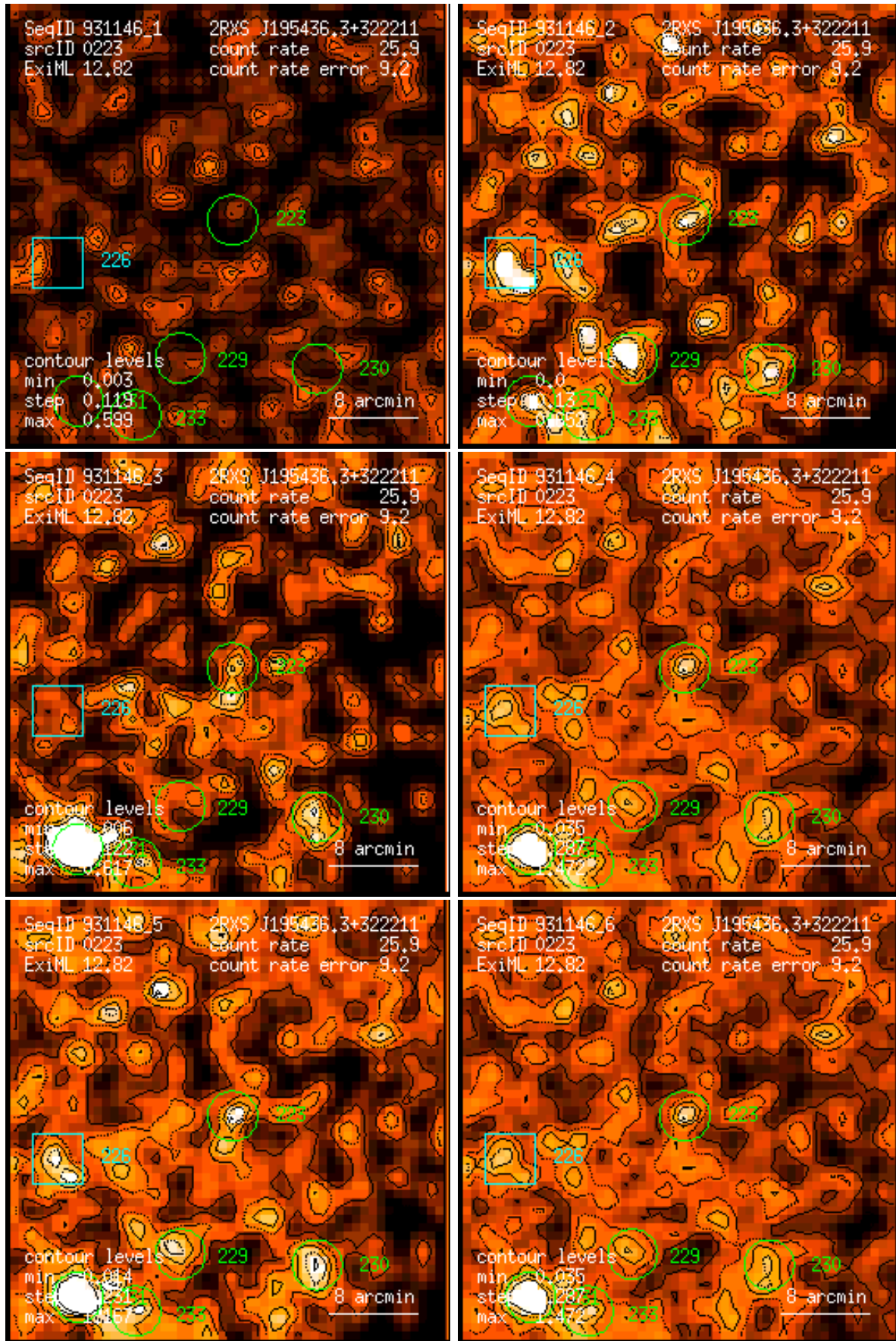
Figure 223: RASS 931146: detection 0223: band rate images, Gaussian filter: (1) PSPC channels 11 – 41, (2) 52 – 90, (3) 91 – 201, (4) 11 – 235, (5) 52 – 201, (6) 11 – 201. Broad band rates in counts/ks. Band rate contour levels in counts/ks/arcmin 2 .
