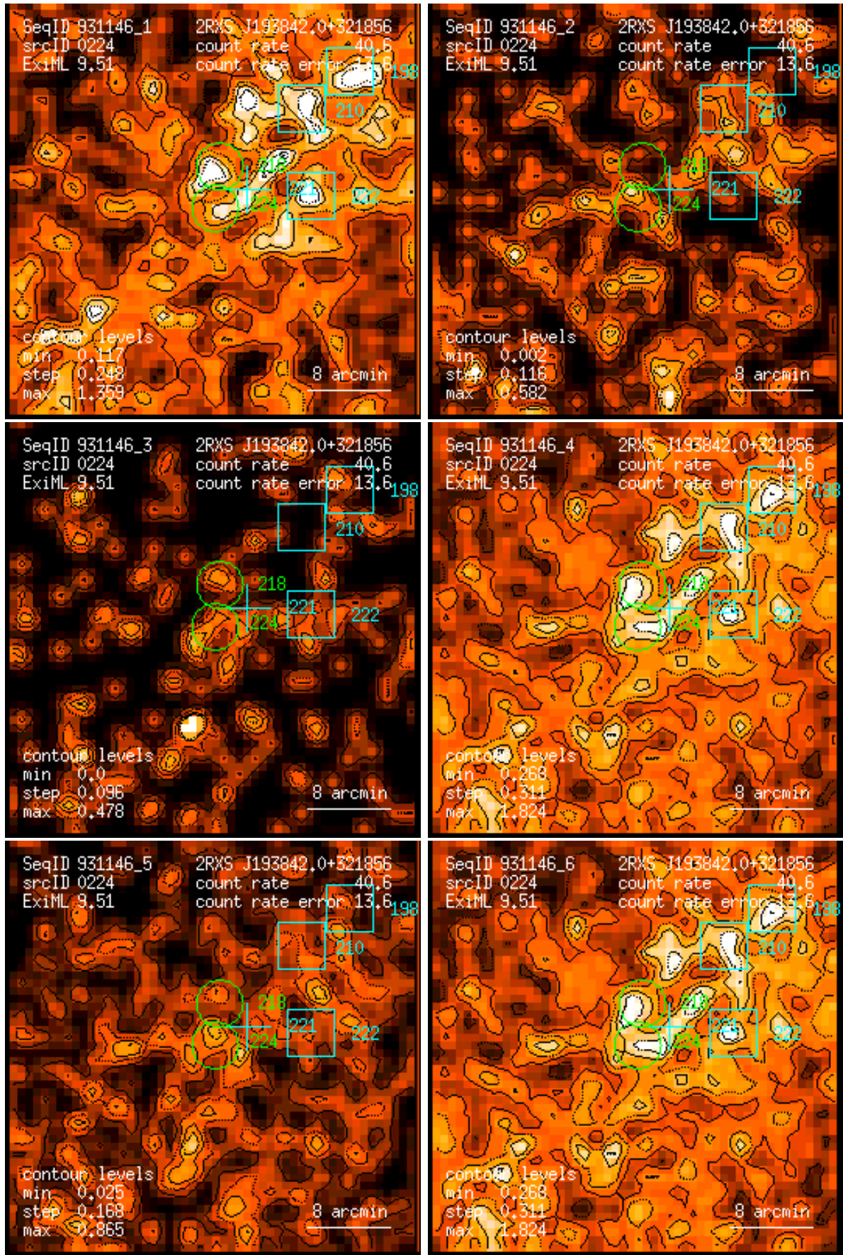
Figure 224: RASS 931146: detection 0224: band rate images, Gaussian filter: (1) PSPC channels 11 – 41, (2) 52 – 90, (3) 91 – 201, (4) 11 – 235, (5) 52 – 201, (6) 11 – 201. Broad band rates in counts/ks. Band rate contour levels in counts/ks/arcmin 2 .
