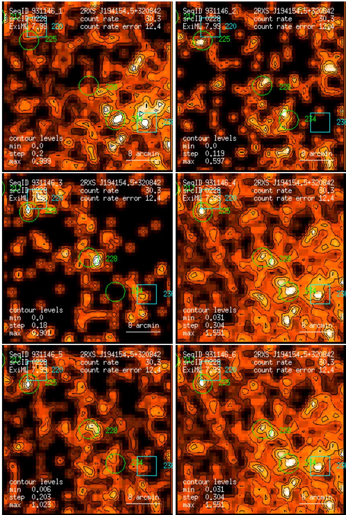
Figure 228: RASS 931146: detection 0228: band rate images, Gaussian filter: (1) PSPC channels 11 – 41, (2) 52 – 90, (3) 91 – 201, (4) 11 – 235, (5) 52 – 201, (6) 11 – 201. Broad band rates in counts/ks. Band rate contour levels in counts/ks/arcmin 2 .
