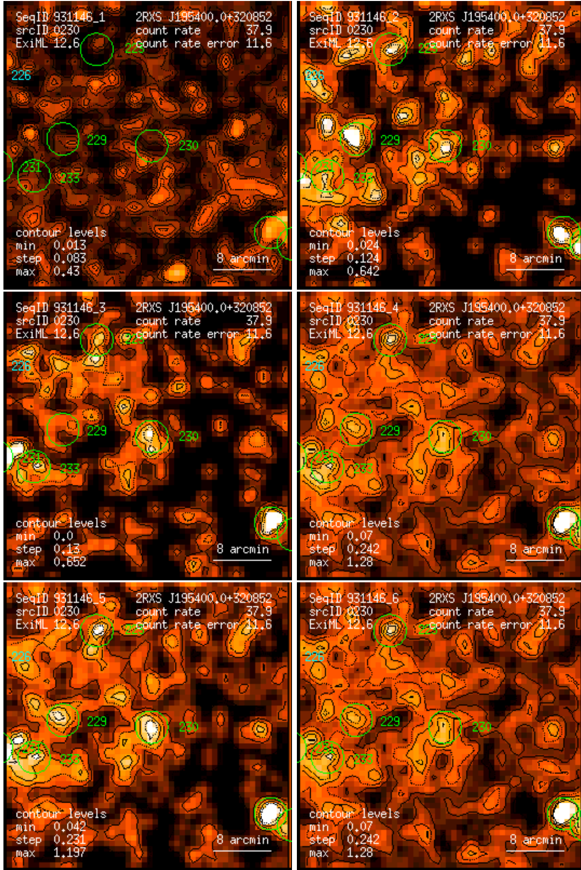
Figure 230: RASS 931146: detection 0230: band rate images, Gaussian filter: (1) PSPC channels 11 – 41, (2) 52 – 90, (3) 91 – 201, (4) 11 – 235, (5) 52 – 201, (6) 11 – 201. Broad band rates in counts/ks. Band rate contour levels in counts/ks/arcmin 2 .
