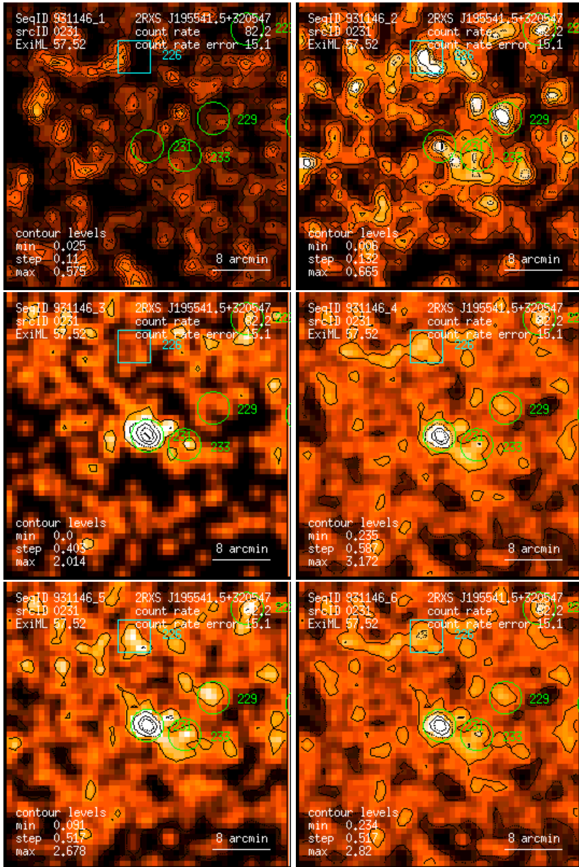
Figure 231: RASS 931146: detection 0231: band rate images, Gaussian filter: (1) PSPC channels 11 – 41, (2) 52 – 90, (3) 91 – 201, (4) 11 – 235, (5) 52 – 201, (6) 11 – 201. Broad band rates in counts/ks. Band rate contour levels in counts/ks/arcmin 2 .
