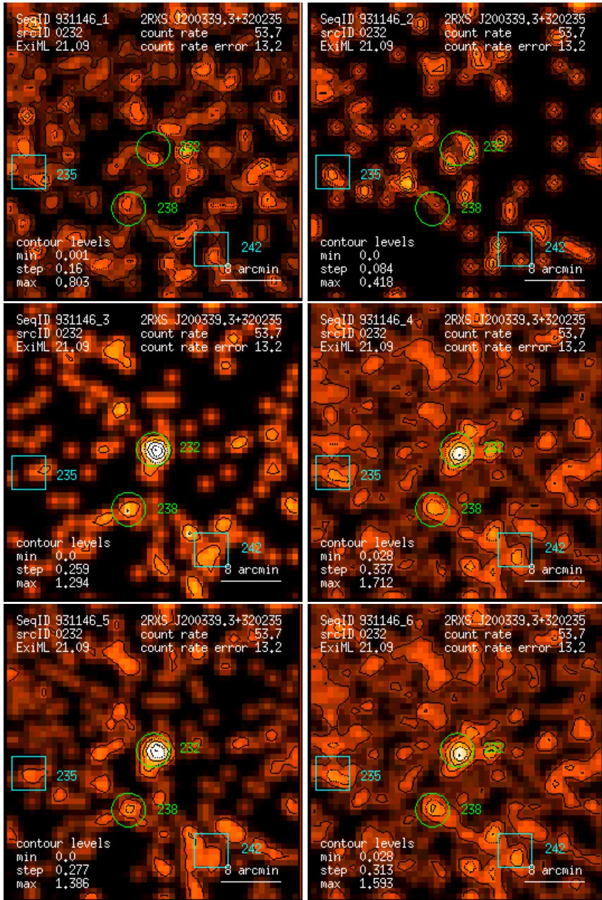
Figure 232: RASS 931146: detection 0232: band rate images, Gaussian filter: (1) PSPC channels 11 – 41, (2) 52 – 90, (3) 91 – 201, (4) 11 – 235, (5) 52 – 201, (6) 11 – 201. Broad band rates in counts/ks. Band rate contour levels in counts/ks/arcmin 2 .
