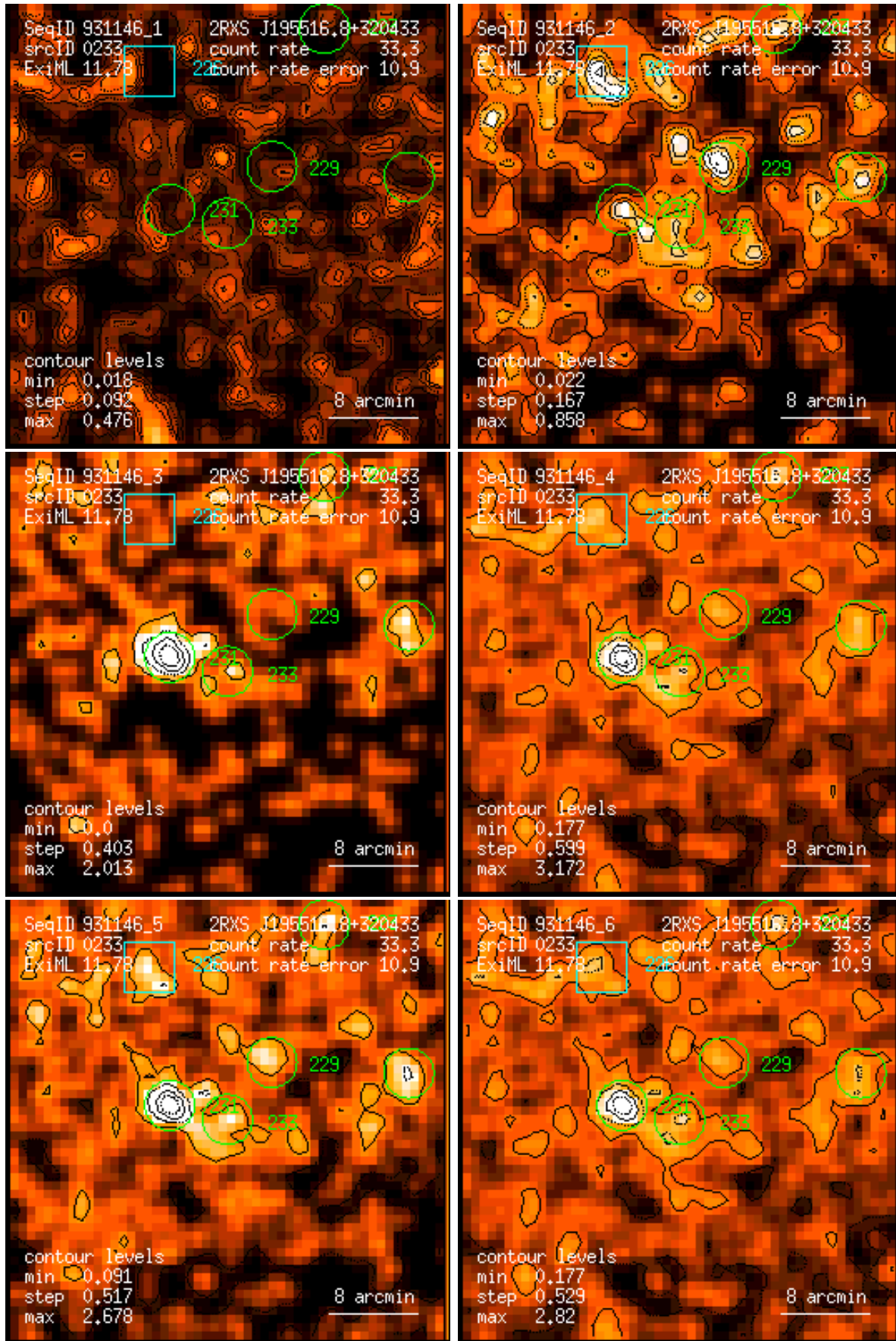
Figure 233: RASS 931146: detection 0233: band rate images, Gaussian filter: (1) PSPC channels 11 – 41, (2) 52 – 90, (3) 91 – 201, (4) 11 – 235, (5) 52 – 201, (6) 11 – 201. Broad band rates in counts/ks. Band rate contour levels in counts/ks/arcmin 2 .
