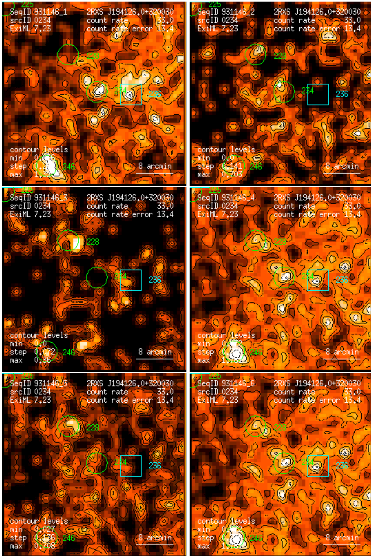
Figure 234: RASS 931146: detection 0234: band rate images, Gaussian filter: (1) PSPC channels 11 – 41, (2) 52 – 90, (3) 91 – 201, (4) 11 – 235, (5) 52 – 201, (6) 11 – 201. Broad band rates in counts/ks. Band rate contour levels in counts/ks/arcmin 2 .
