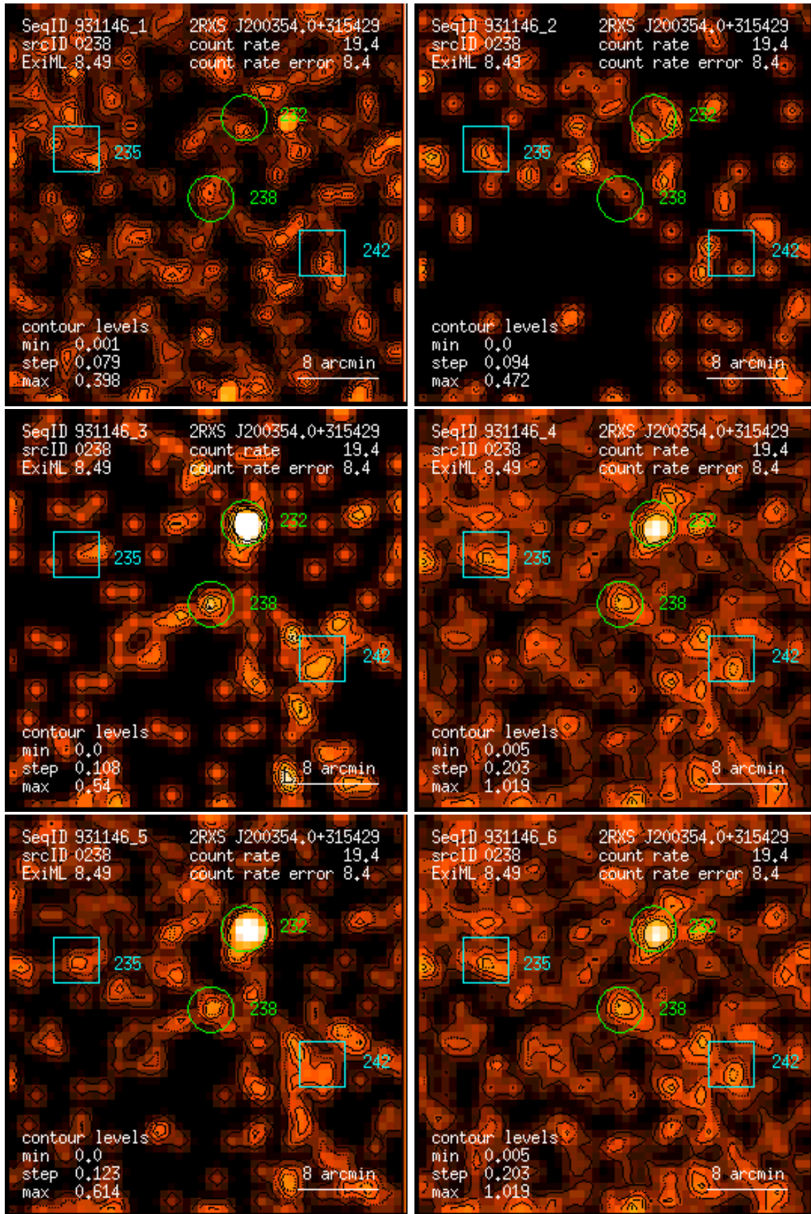
Figure 238: RASS 931146: detection 0238: band rate images, Gaussian filter: (1) PSPC channels 11 – 41, (2) 52 – 90, (3) 91 – 201, (4) 11 – 235, (5) 52 – 201, (6) 11 – 201. Broad band rates in counts/ks. Band rate contour levels in counts/ks/arcmin 2 .
