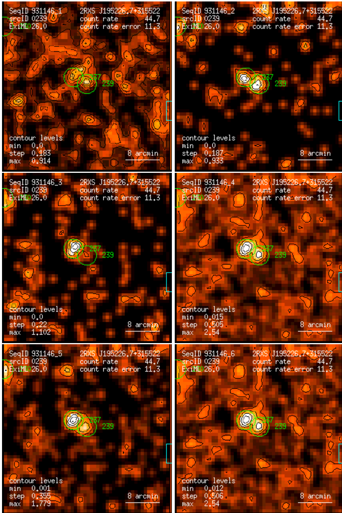
Figure 239: RASS 931146: detection 0239: band rate images, Gaussian filter: (1) PSPC channels 11 – 41, (2) 52 – 90, (3) 91 – 201, (4) 11 – 235, (5) 52 – 201, (6) 11 – 201. Broad band rates in counts/ks. Band rate contour levels in counts/ks/arcmin 2 .
