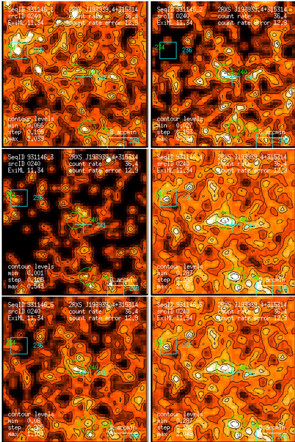
Figure 240: RASS 931146: detection 0240: band rate images, Gaussian filter: (1) PSPC channels 11 – 41, (2) 52 – 90, (3) 91 – 201, (4) 11 – 235, (5) 52 – 201, (6) 11 – 201. Broad band rates in counts/ks. Band rate contour levels in counts/ks/arcmin 2 .
