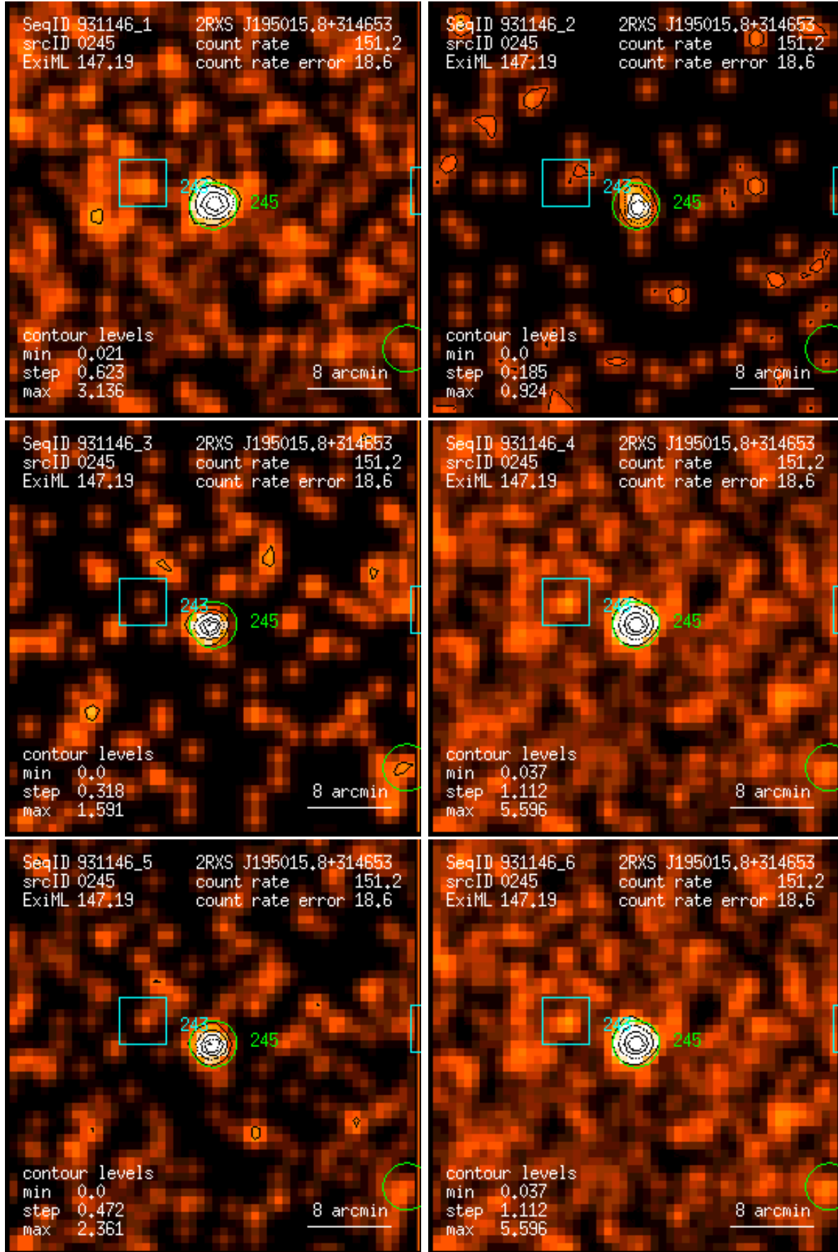
Figure 245: RASS 931146: detection 0245: band rate images, Gaussian filter: (1) PSPC channels 11 – 41, (2) 52 – 90, (3) 91 – 201, (4) 11 – 235, (5) 52 – 201, (6) 11 – 201. Broad band rates in counts/ks. Band rate contour levels in counts/ks/arcmin 2 .
