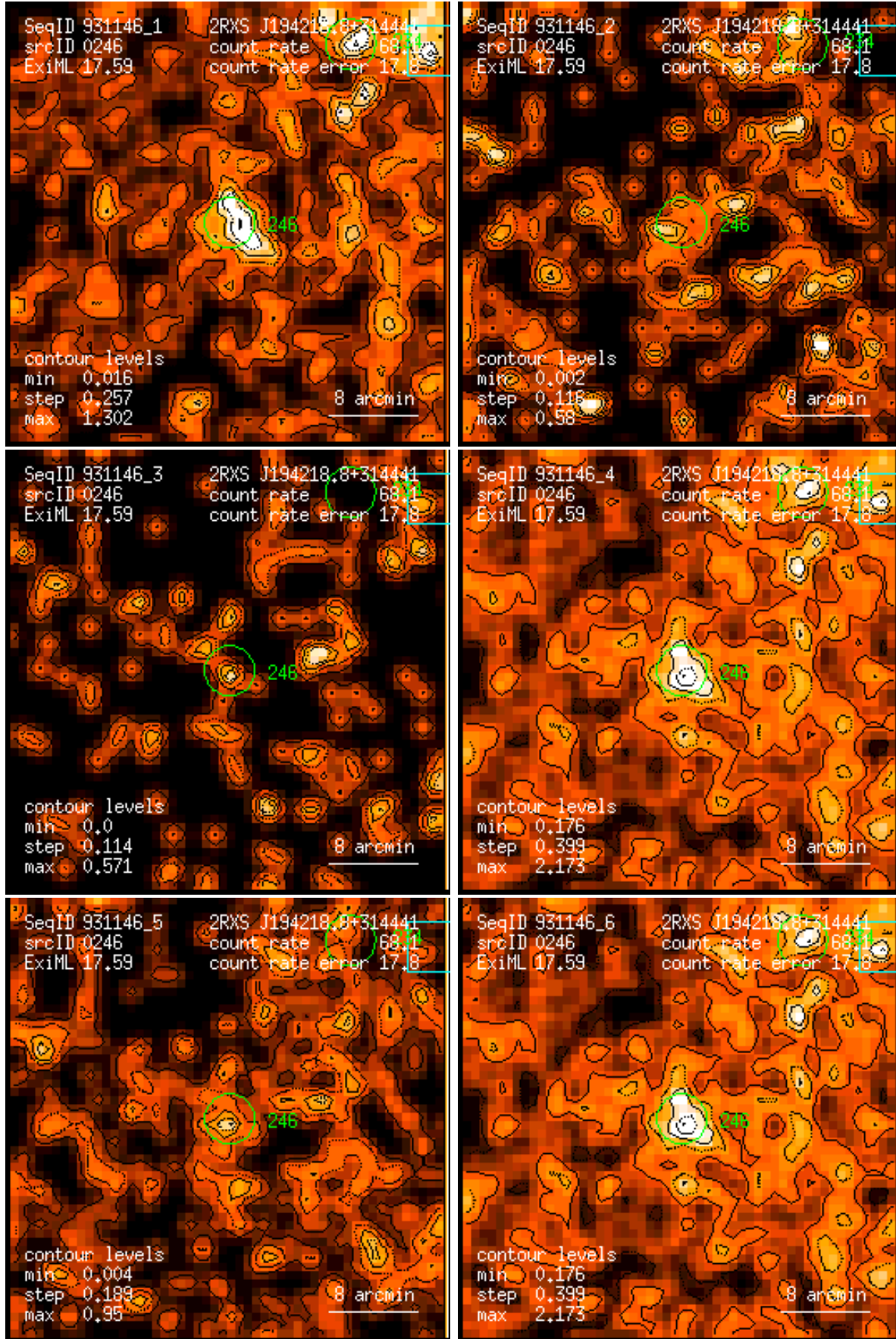
Figure 246: RASS 931146: detection 0246: band rate images, Gaussian filter: (1) PSPC channels 11 – 41, (2) 52 – 90, (3) 91 – 201, (4) 11 – 235, (5) 52 – 201, (6) 11 – 201. Broad band rates in counts/ks. Band rate contour levels in counts/ks/arcmin 2 .
