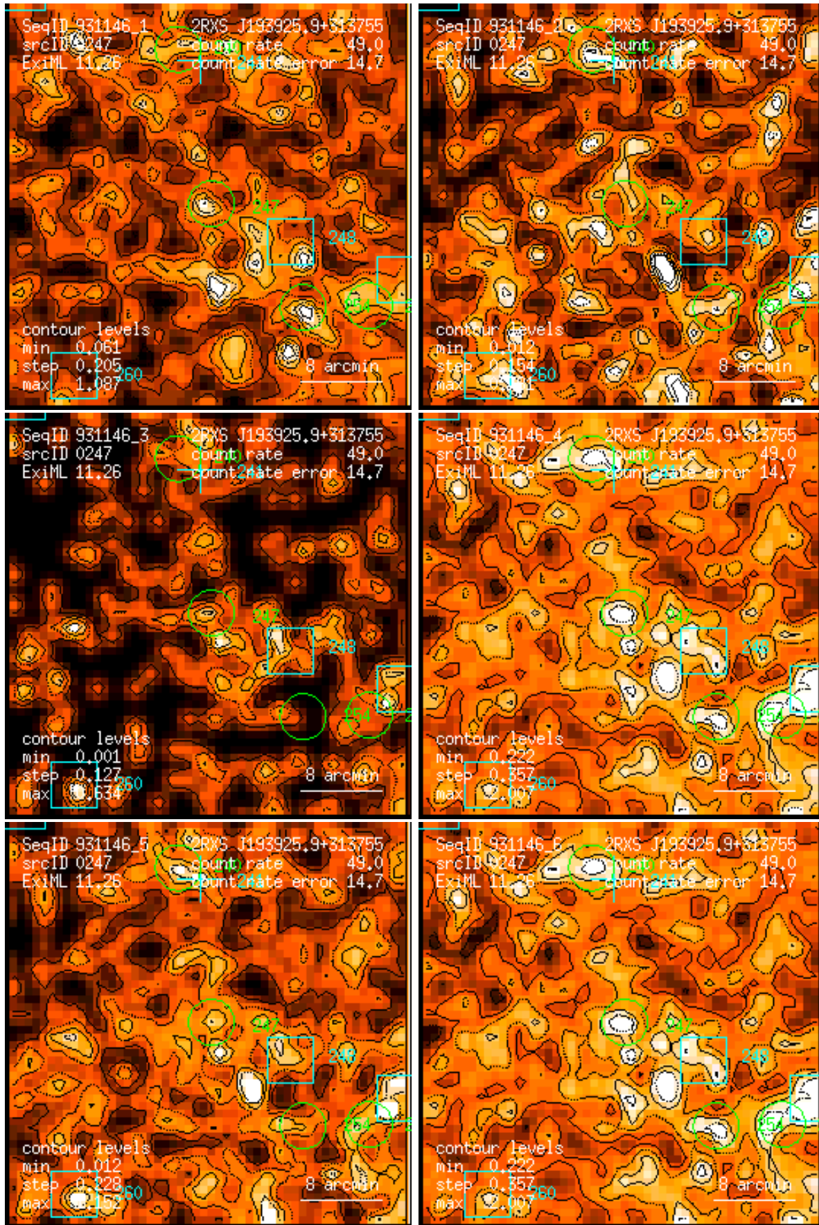
Figure 247: RASS 931146: detection 0247: band rate images, Gaussian filter: (1) PSPC channels 11 – 41, (2) 52 – 90, (3) 91 – 201, (4) 11 – 235, (5) 52 – 201, (6) 11 – 201. Broad band rates in counts/ks. Band rate contour levels in counts/ks/arcmin 2 .
