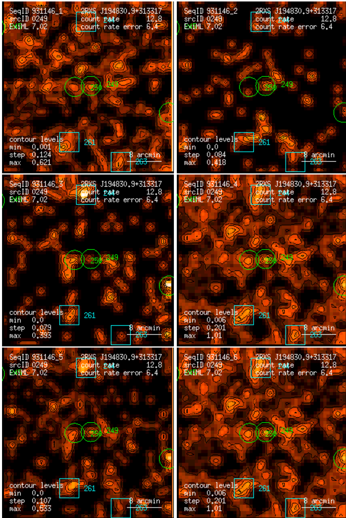
Figure 249: RASS 931146: detection 0249: band rate images, Gaussian filter: (1) PSPC channels 11 – 41, (2) 52 – 90, (3) 91 – 201, (4) 11 – 235, (5) 52 – 201, (6) 11 – 201. Broad band rates in counts/ks. Band rate contour levels in counts/ks/arcmin 2 .
