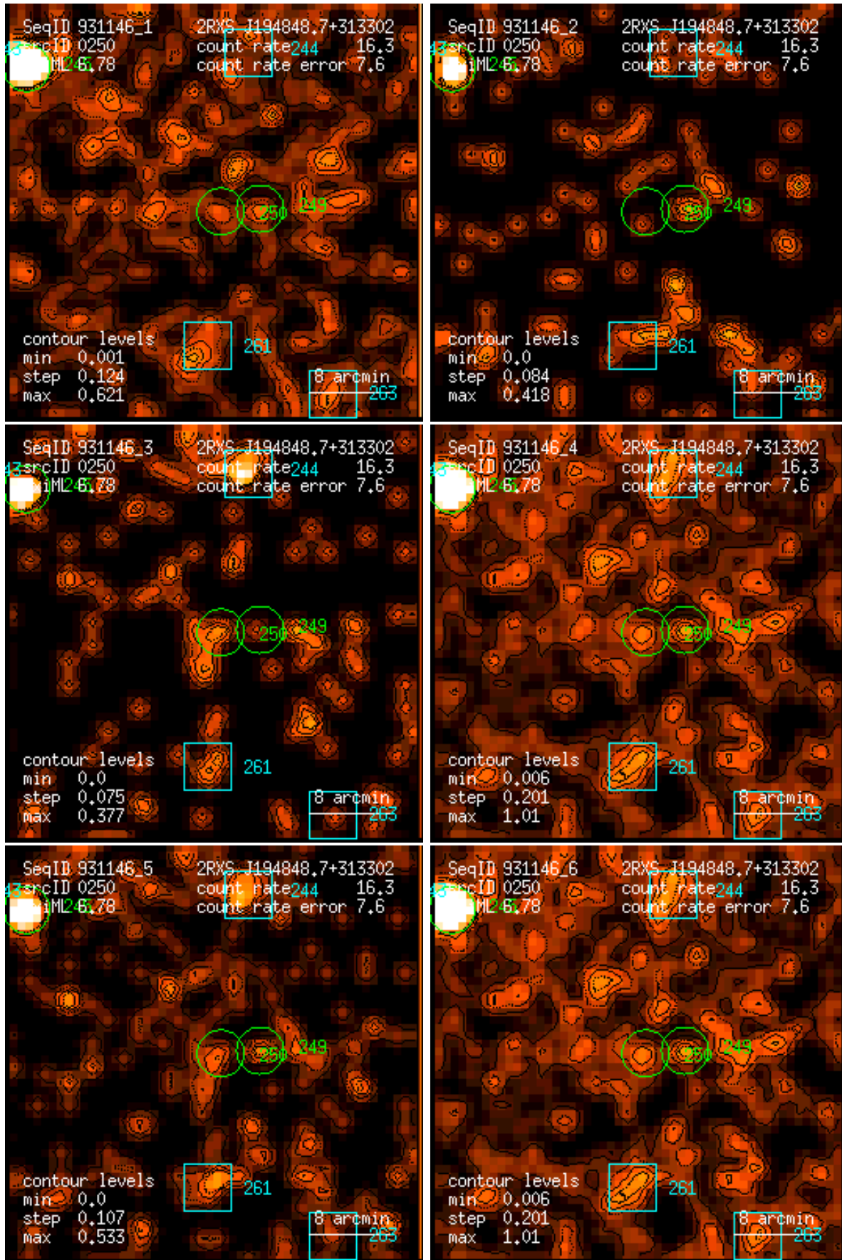
Figure 250: RASS 931146: detection 0250: band rate images, Gaussian filter: (1) PSPC channels 11 – 41, (2) 52 – 90, (3) 91 – 201, (4) 11 – 235, (5) 52 – 201, (6) 11 – 201. Broad band rates in counts/ks. Band rate contour levels in counts/ks/arcmin 2 .
