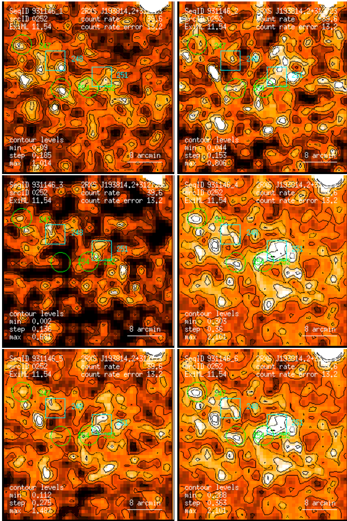
Figure 252: RASS 931146: detection 0252: band rate images, Gaussian filter: (1) PSPC channels 11 – 41, (2) 52 – 90, (3) 91 – 201, (4) 11 – 235, (5) 52 – 201, (6) 11 – 201. Broad band rates in counts/ks. Band rate contour levels in counts/ks/arcmin 2 .
