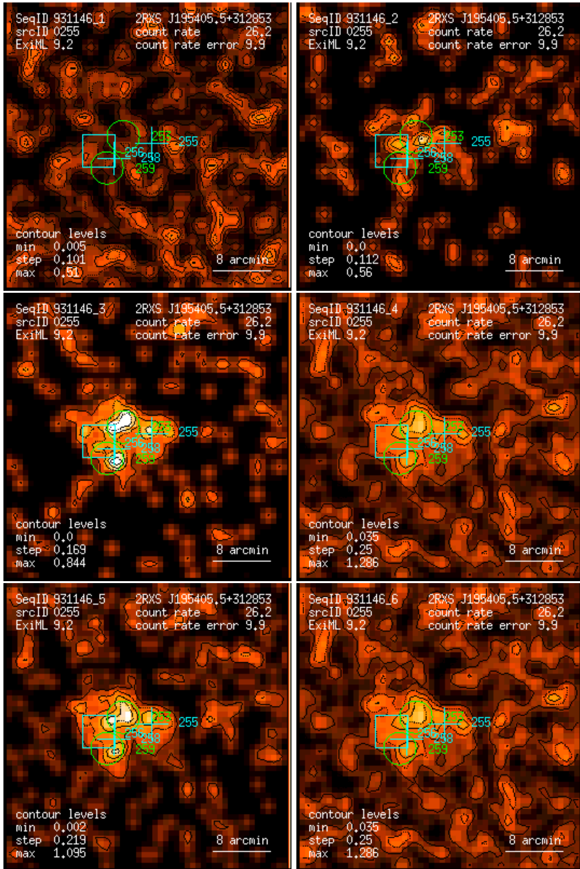
Figure 255: RASS 931146: detection 0255: band rate images, Gaussian filter: (1) PSPC channels 11 – 41, (2) 52 – 90, (3) 91 – 201, (4) 11 – 235, (5) 52 – 201, (6) 11 – 201. Broad band rates in counts/ks. Band rate contour levels in counts/ks/arcmin 2 .
