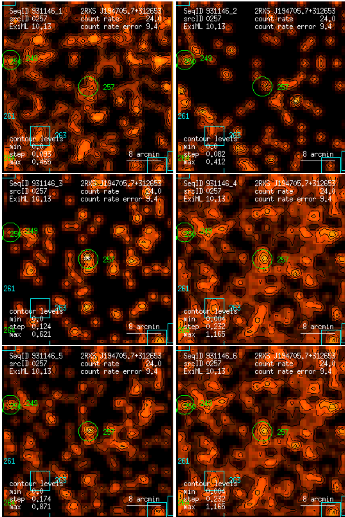
Figure 257: RASS 931146: detection 0257: band rate images, Gaussian filter: (1) PSPC channels 11 – 41, (2) 52 – 90, (3) 91 – 201, (4) 11 – 235, (5) 52 – 201, (6) 11 – 201. Broad band rates in counts/ks. Band rate contour levels in counts/ks/arcmin 2 .
