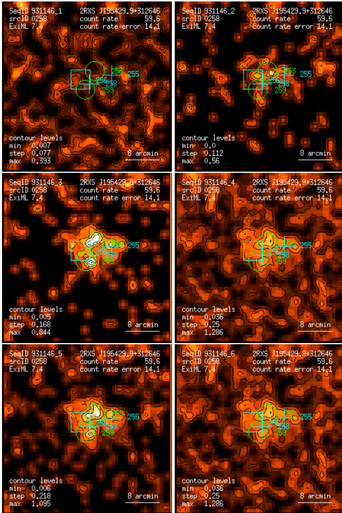
Figure 258: RASS 931146: detection 0258: band rate images, Gaussian filter: (1) PSPC channels 11 – 41, (2) 52 – 90, (3) 91 – 201, (4) 11 – 235, (5) 52 – 201, (6) 11 – 201. Broad band rates in counts/ks. Band rate contour levels in counts/ks/arcmin 2 .
